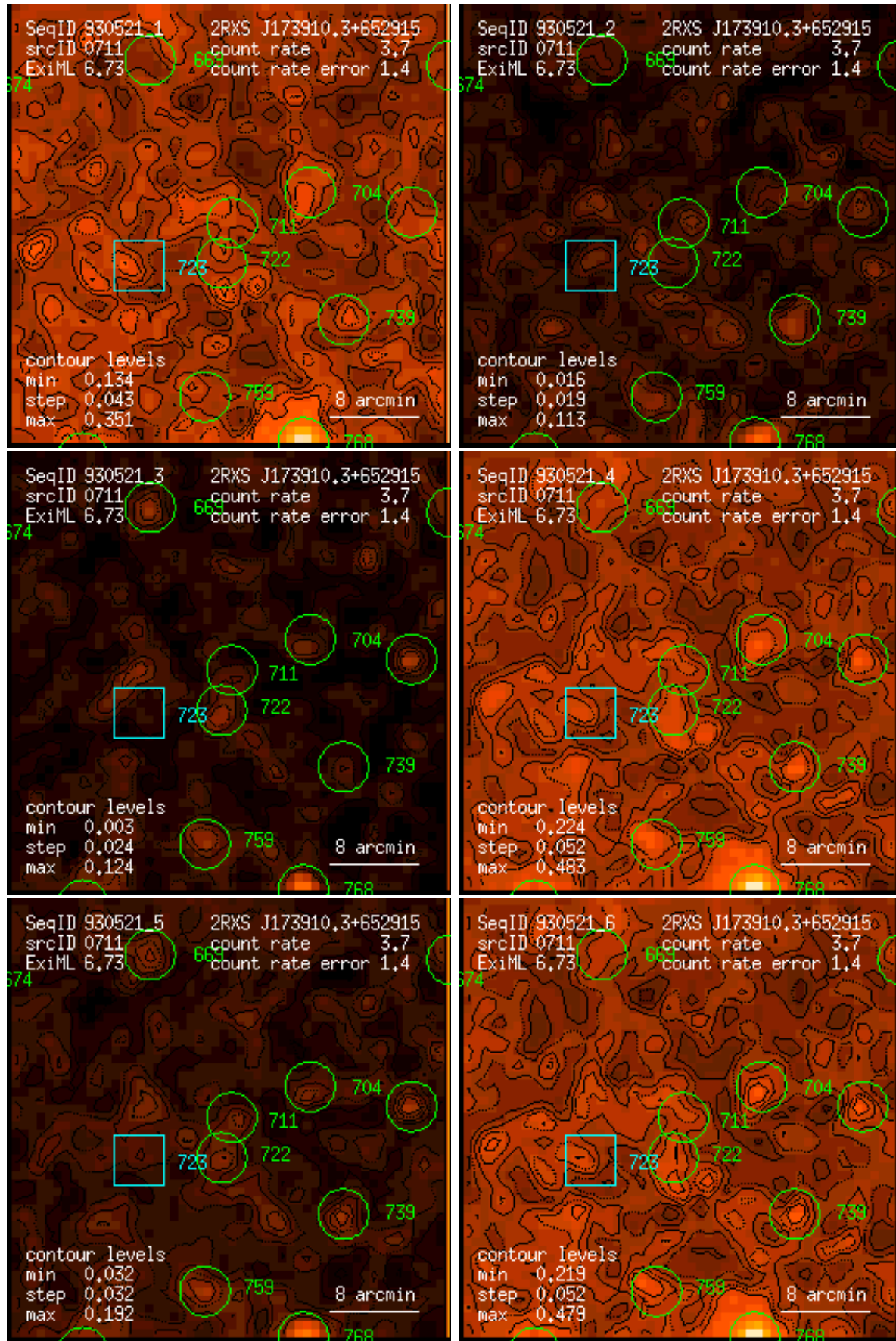
Figure 711: RASS 930521: detection 0711: band rate images, Gaussian filter: (1) PSPC channels 11 – 41, (2) 52 – 90, (3) 91 – 201, (4) 11 – 235, (5) 52 – 201, (6) 11 – 201. Broad band rates in counts/ks. Band rate contour levels in counts/ks/arcmin 2 .
