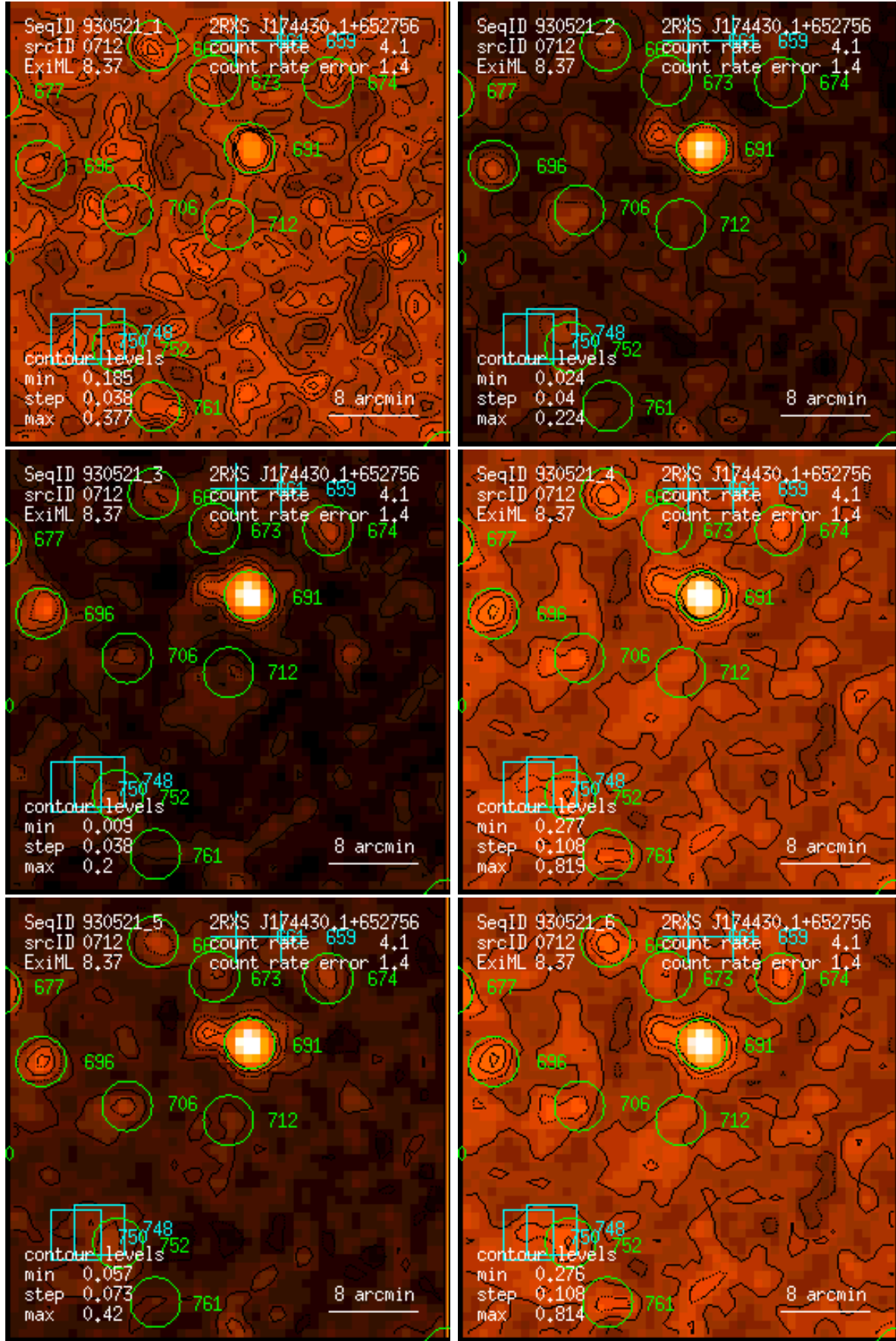
Figure 712: RASS 930521: detection 0712: band rate images, Gaussian filter: (1) PSPC channels 11 – 41, (2) 52 – 90, (3) 91 – 201, (4) 11 – 235, (5) 52 – 201, (6) 11 – 201. Broad band rates in counts/ks. Band rate contour levels in counts/ks/arcmin 2 .
