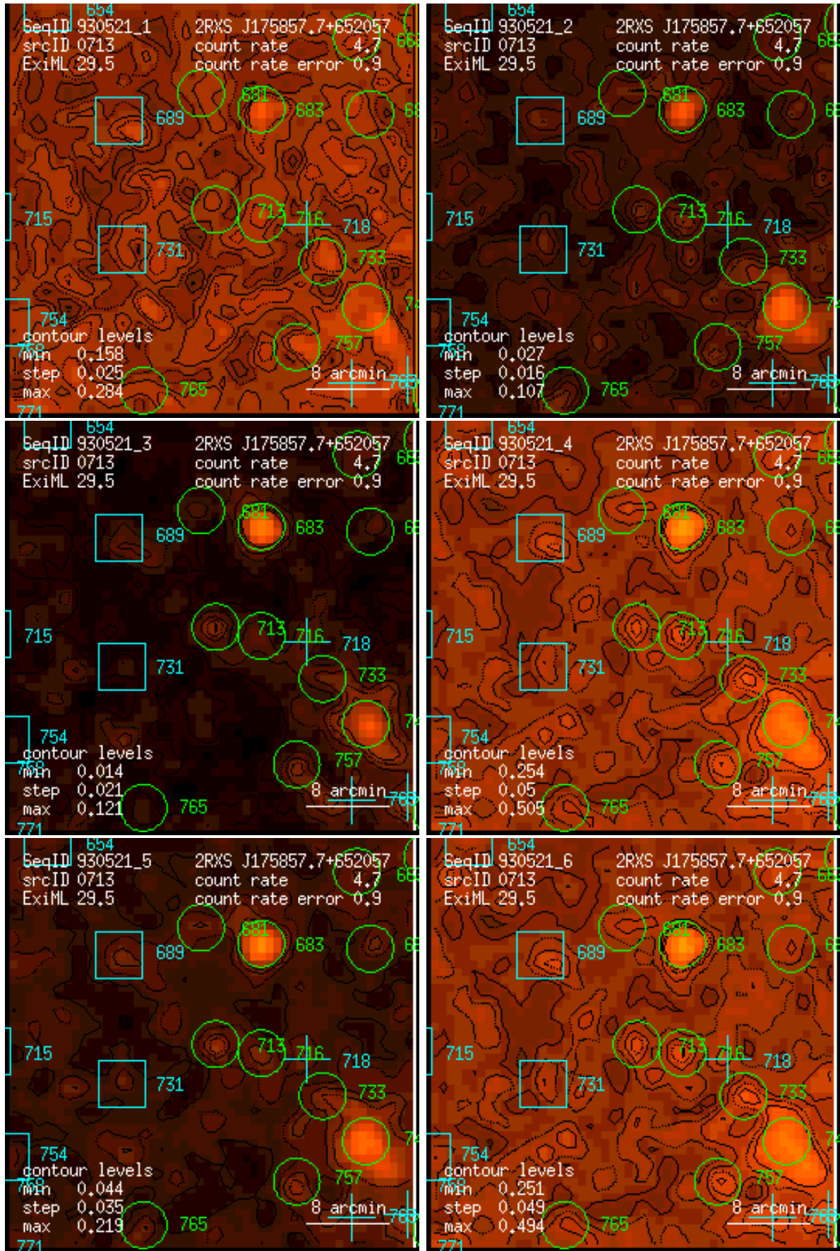
Figure 713: RASS 930521: detection 0713: band rate images, Gaussian filter: (1) PSPC channels 11 – 41, (2) 52 – 90, (3) 91 – 201, (4) 11 – 235, (5) 52 – 201, (6) 11 – 201. Broad band rates in counts/ks. Band rate contour levels in counts/ks/arcmin 2 .
