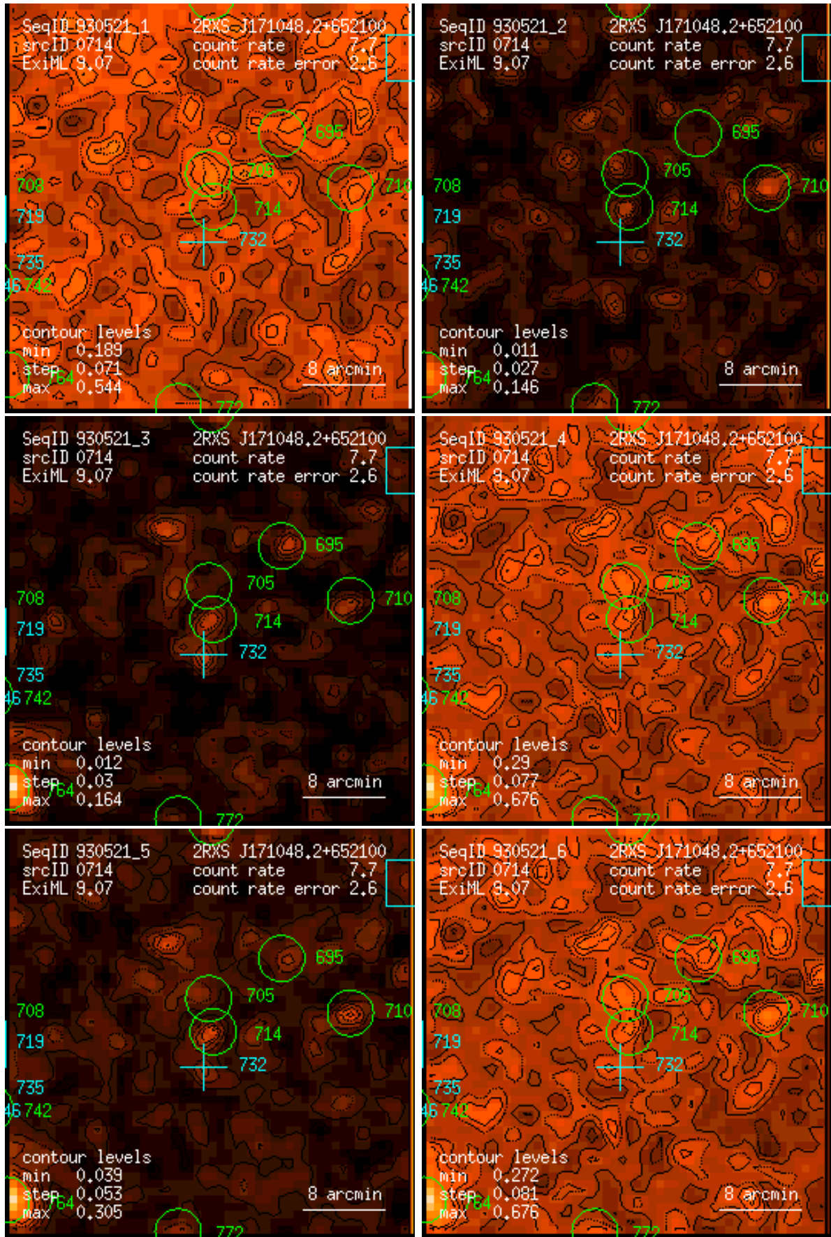
Figure 714: RASS 930521: detection 0714: band rate images, Gaussian filter: (1) PSPC channels 11 – 41, (2) 52 – 90, (3) 91 – 201, (4) 11 – 235, (5) 52 – 201, (6) 11 – 201. Broad band rates in counts/ks. Band rate contour levels in counts/ks/arcmin 2 .
