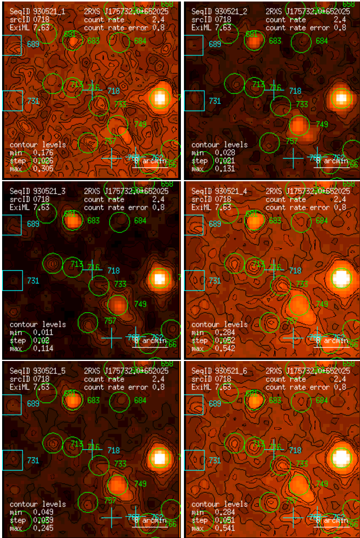
Figure 718: RASS 930521: detection 0718: band rate images, Gaussian filter: (1) PSPC channels 11 – 41, (2) 52 – 90, (3) 91 – 201, (4) 11 – 235, (5) 52 – 201, (6) 11 – 201. Broad band rates in counts/ks. Band rate contour levels in counts/ks/arcmin 2 .
