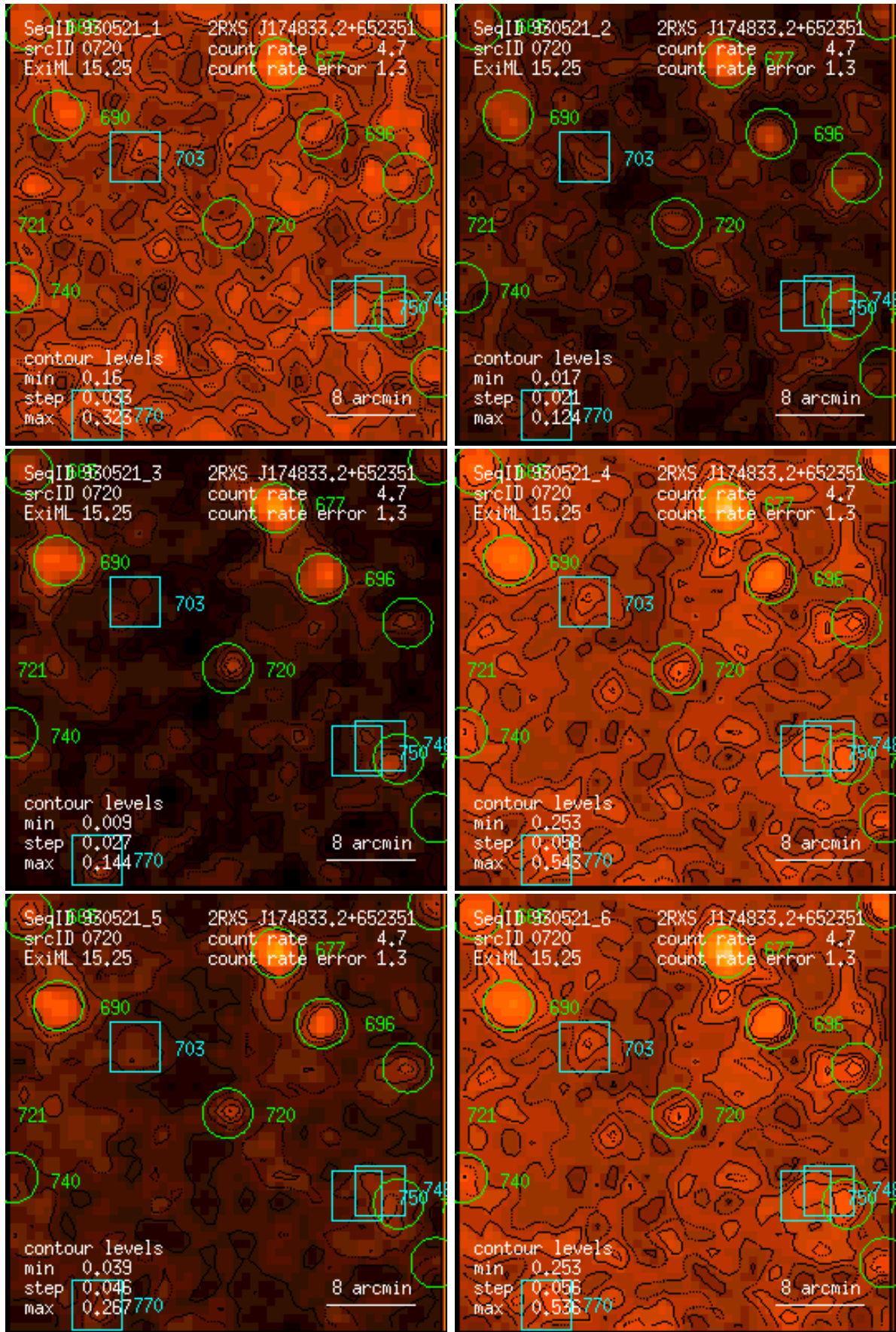
Figure 720: RASS 930521: detection 0720: band rate images, Gaussian filter: (1) PSPC channels 11 – 41, (2) 52 – 90, (3) 91 – 201, (4) 11 – 235, (5) 52 – 201, (6) 11 – 201. Broad band rates in counts/ks. Band rate contour levels in counts/ks/arcmin 2 .
