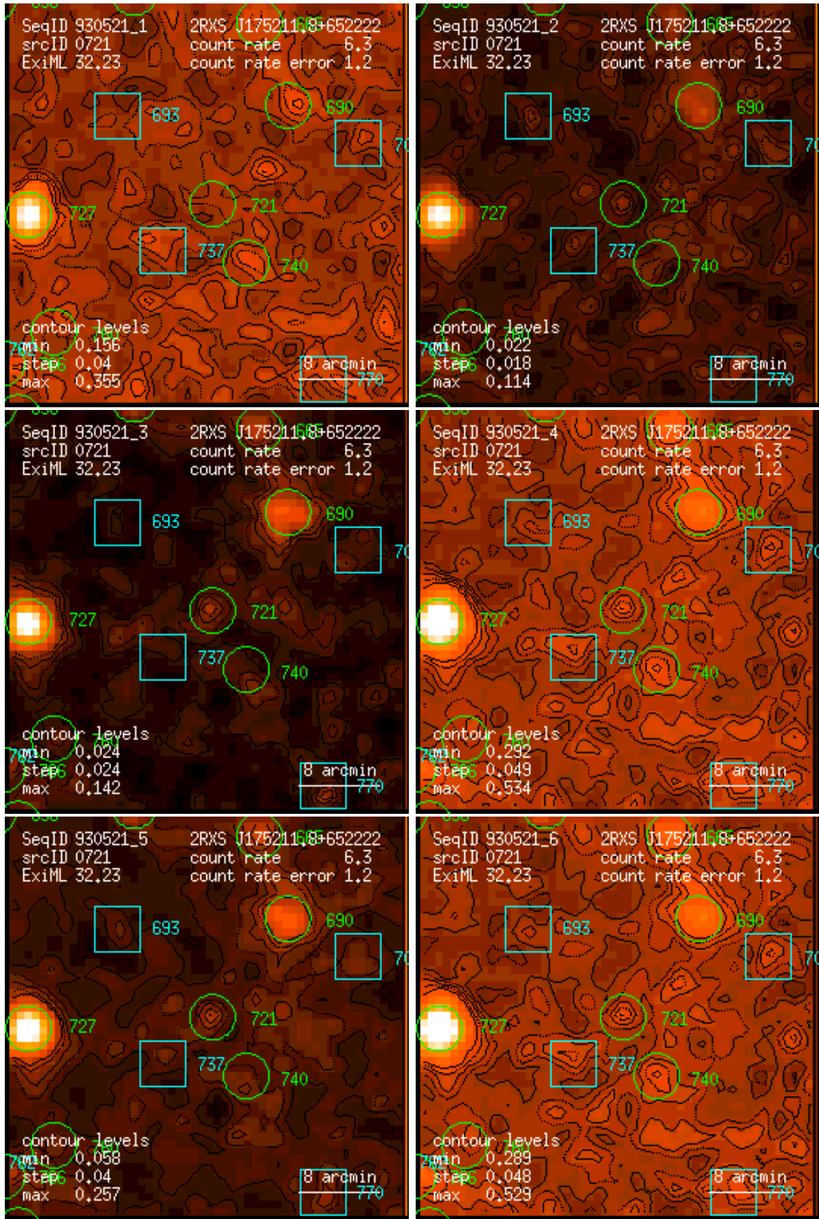
Figure 721: RASS 930521: detection 0721: band rate images, Gaussian filter: (1) PSPC channels 11 – 41, (2) 52 – 90, (3) 91 – 201, (4) 11 – 235, (5) 52 – 201, (6) 11 – 201. Broad band rates in counts/ks. Band rate contour levels in counts/ks/arcmin 2 .
