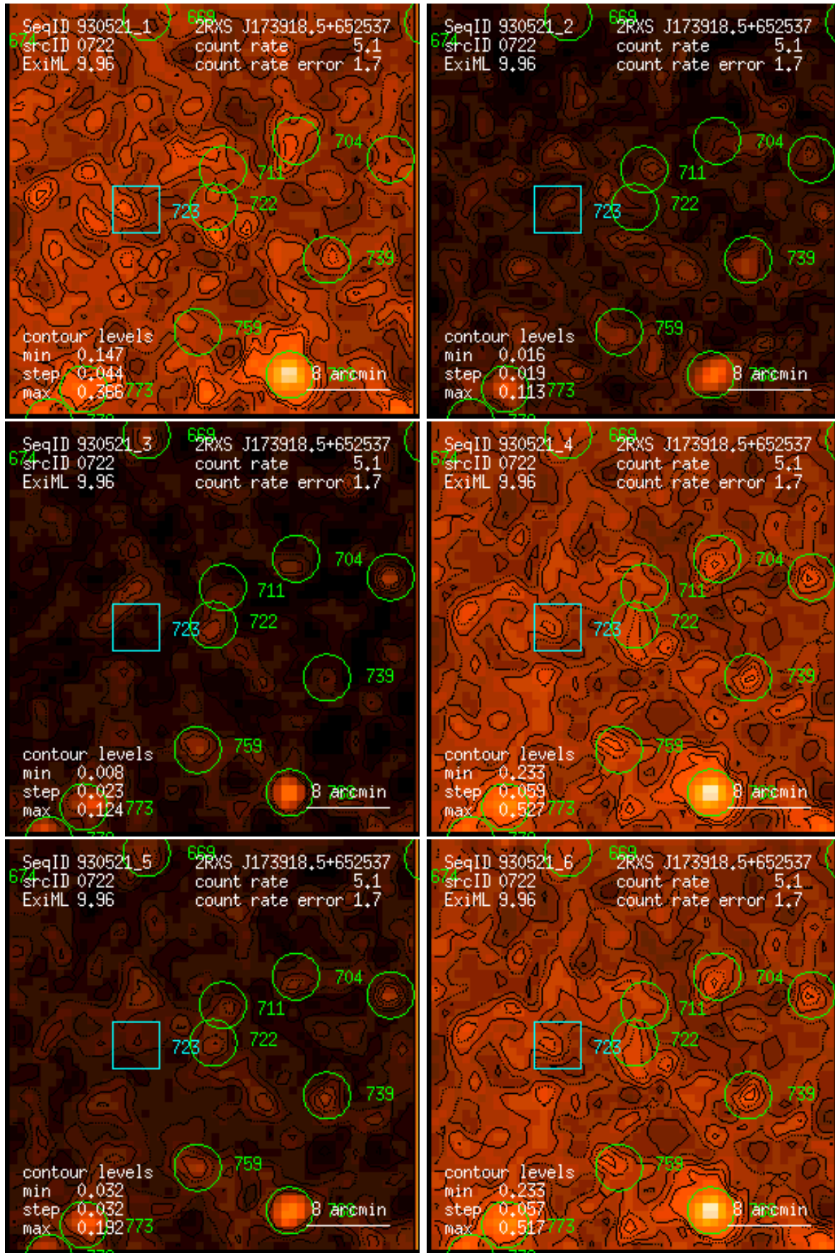
Figure 722: RASS 930521: detection 0722: band rate images, Gaussian filter: (1) PSPC channels 11 – 41, (2) 52 – 90, (3) 91 – 201, (4) 11 – 235, (5) 52 – 201, (6) 11 – 201. Broad band rates in counts/ks. Band rate contour levels in counts/ks/arcmin 2 .
