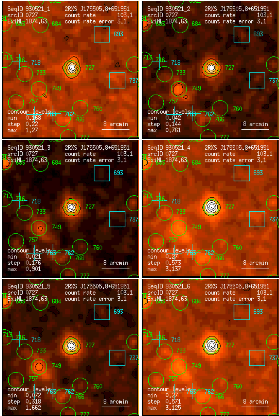
Figure 727: RASS 930521: detection 0727: band rate images, Gaussian filter: (1) PSPC channels 11 – 41, (2) 52 – 90, (3) 91 – 201, (4) 11 – 235, (5) 52 – 201, (6) 11 – 201. Broad band rates in counts/ks. Band rate contour levels in counts/ks/arcmin 2 .
