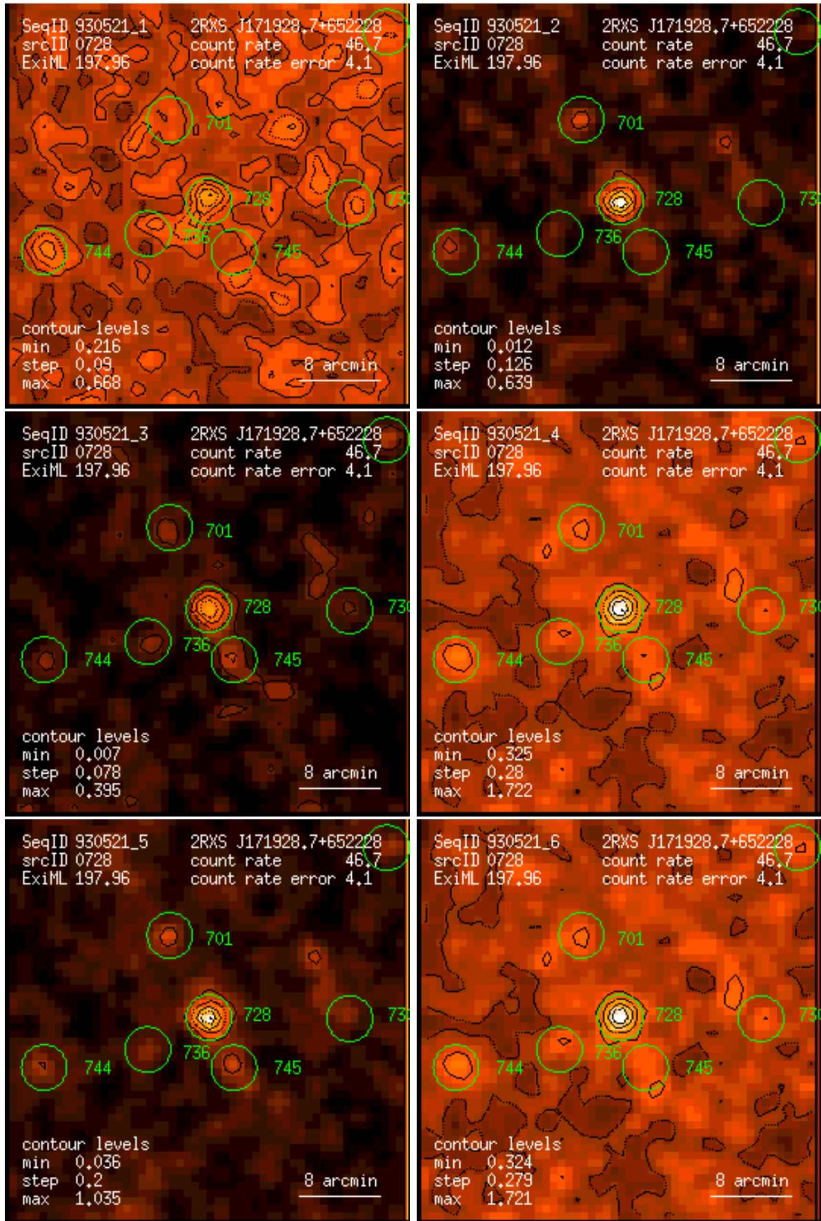
Figure 728: RASS 930521: detection 0728: band rate images, Gaussian filter: (1) PSPC channels 11 – 41, (2) 52 – 90, (3) 91 – 201, (4) 11 – 235, (5) 52 – 201, (6) 11 – 201. Broad band rates in counts/ks. Band rate contour levels in counts/ks/arcmin 2 .
