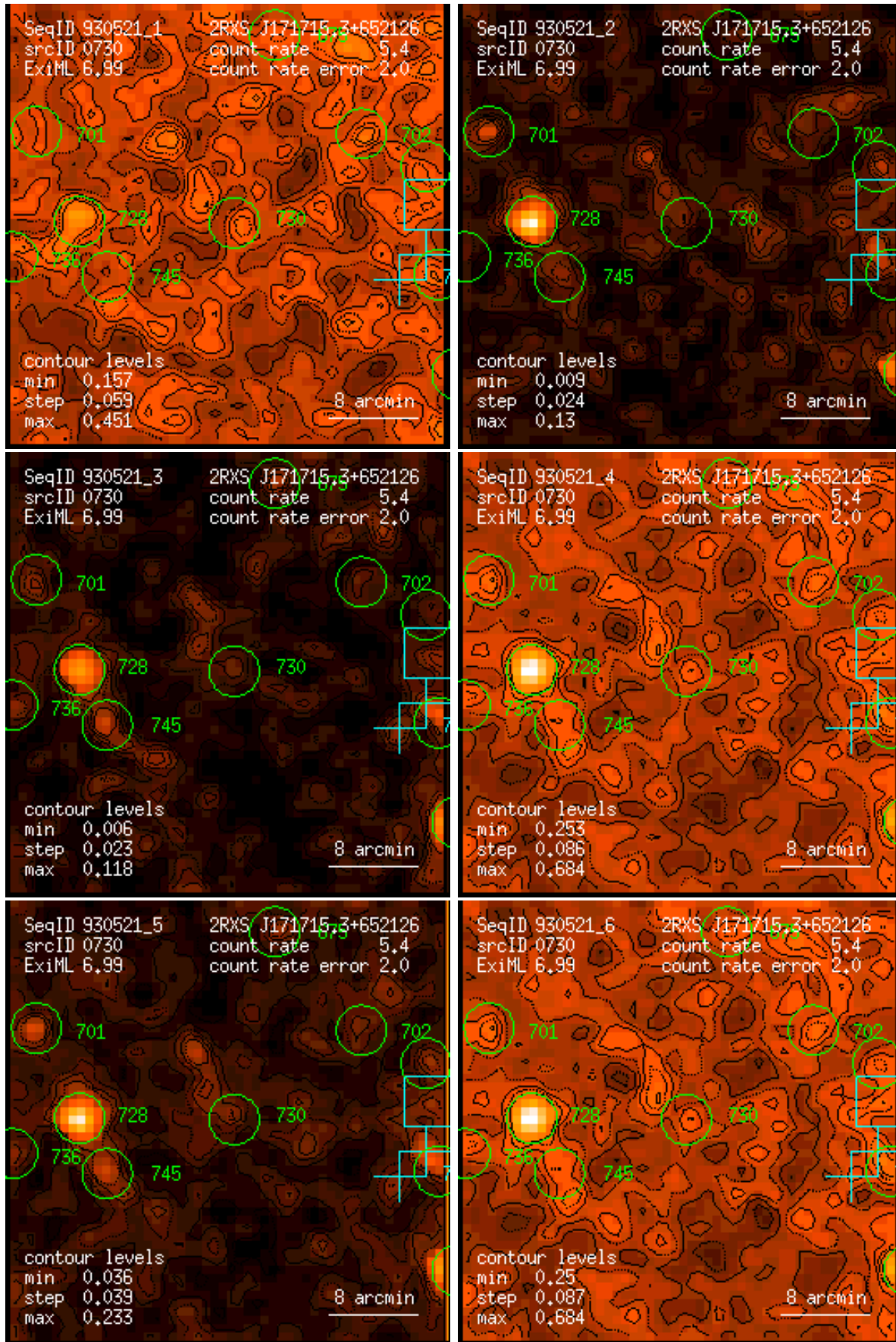
Figure 730: RASS 930521: detection 0730: band rate images, Gaussian filter: (1) PSPC channels 11 – 41, (2) 52 – 90, (3) 91 – 201, (4) 11 – 235, (5) 52 – 201, (6) 11 – 201. Broad band rates in counts/ks. Band rate contour levels in counts/ks/arcmin 2 .
