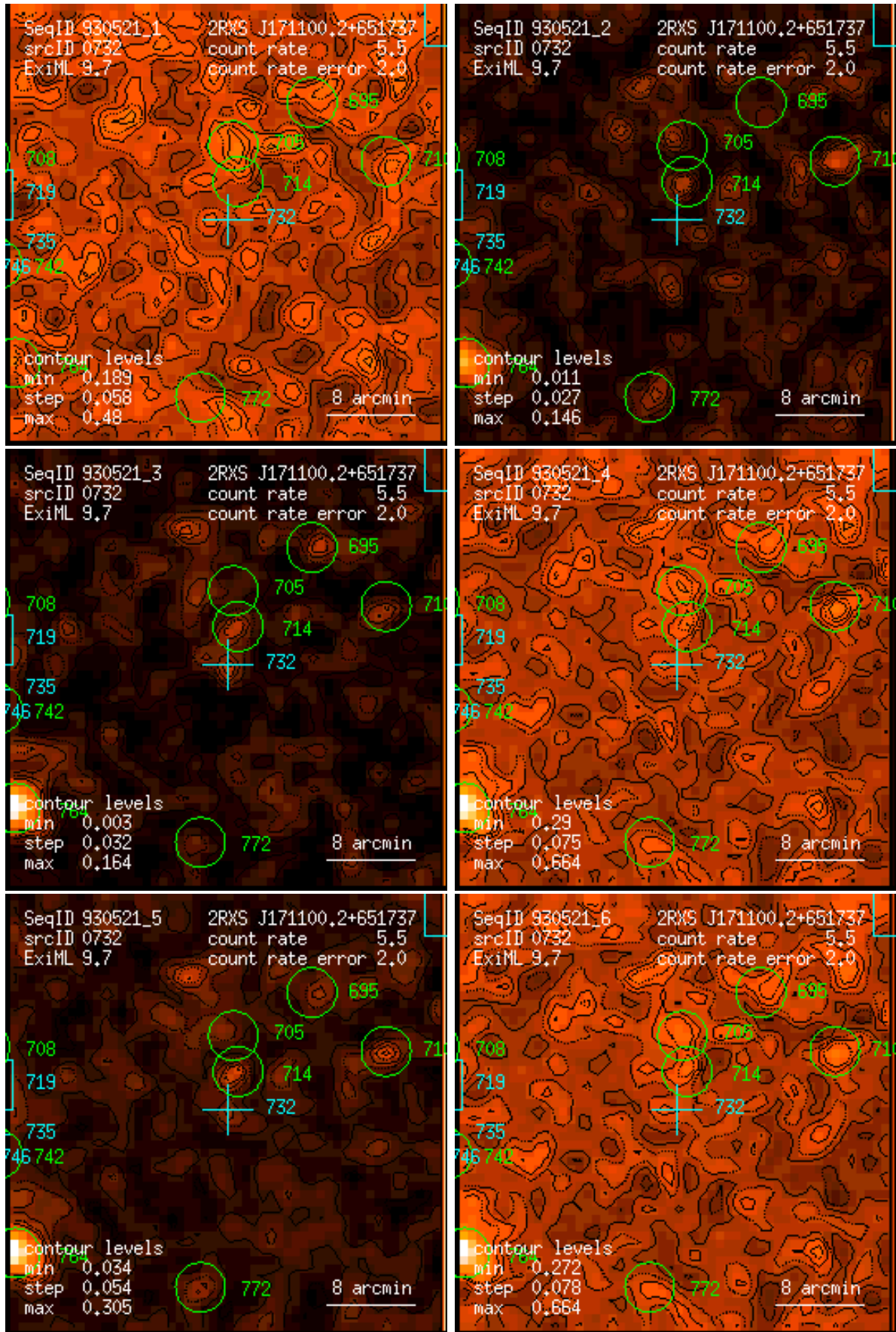
Figure 732: RASS 930521: detection 0732: band rate images, Gaussian filter: (1) PSPC channels 11 – 41, (2) 52 – 90, (3) 91 – 201, (4) 11 – 235, (5) 52 – 201, (6) 11 – 201. Broad band rates in counts/ks. Band rate contour levels in counts/ks/arcmin 2 .
