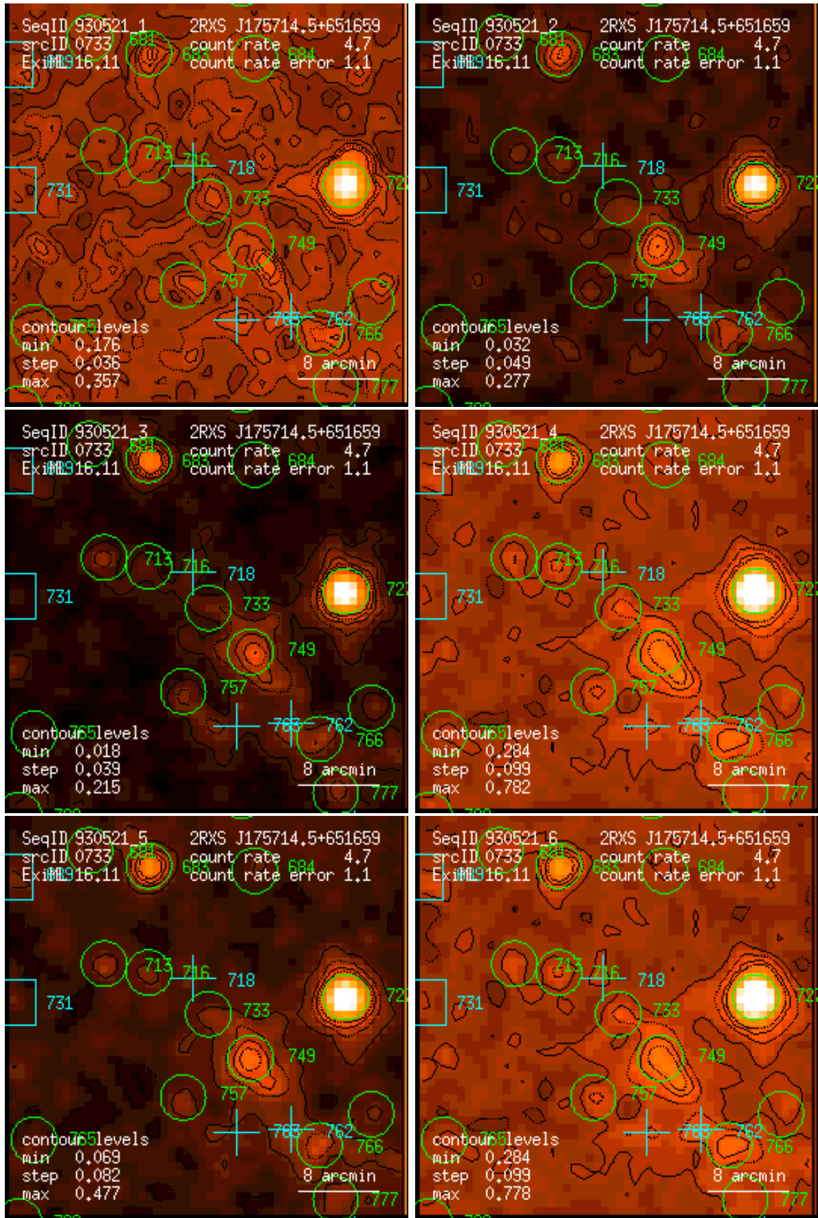
Figure 733: RASS 930521: detection 0733: band rate images, Gaussian filter: (1) PSPC channels 11 – 41, (2) 52 – 90, (3) 91 – 201, (4) 11 – 235, (5) 52 – 201, (6) 11 – 201. Broad band rates in counts/ks. Band rate contour levels in counts/ks/arcmin 2 .
