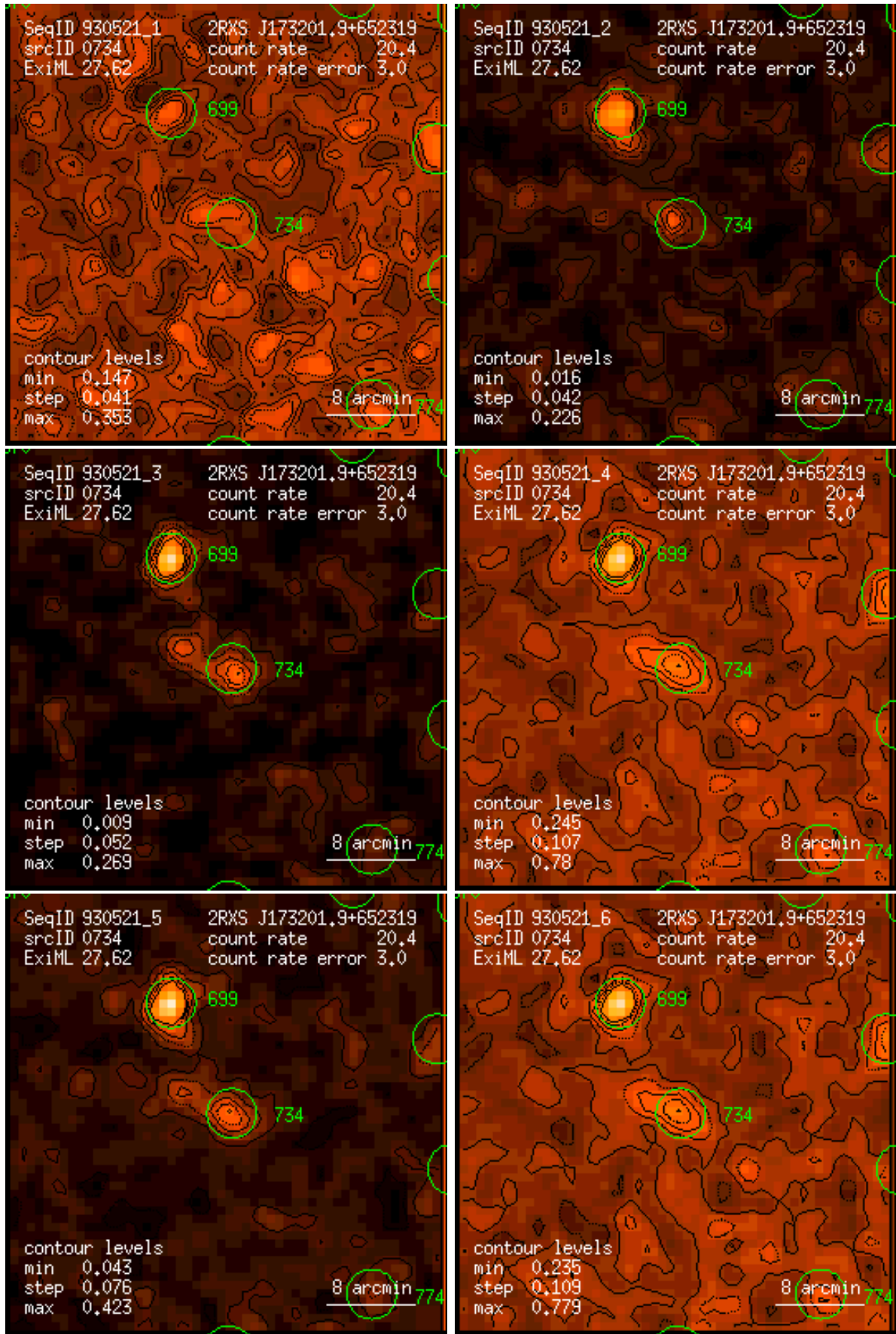
Figure 734: RASS 930521: detection 0734: band rate images, Gaussian filter: (1) PSPC channels 11 – 41, (2) 52 – 90, (3) 91 – 201, (4) 11 – 235, (5) 52 – 201, (6) 11 – 201. Broad band rates in counts/ks. Band rate contour levels in counts/ks/arcmin 2 .
