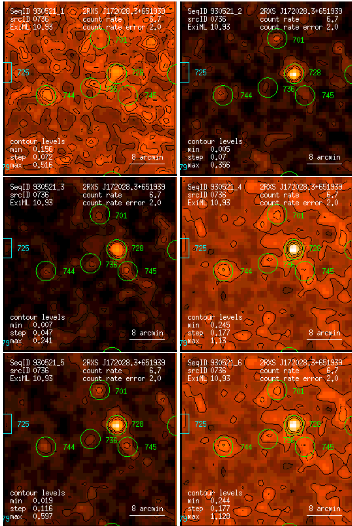
Figure 736: RASS 930521: detection 0736: band rate images, Gaussian filter: (1) PSPC channels 11 – 41, (2) 52 – 90, (3) 91 – 201, (4) 11 – 235, (5) 52 – 201, (6) 11 – 201. Broad band rates in counts/ks. Band rate contour levels in counts/ks/arcmin 2 .
