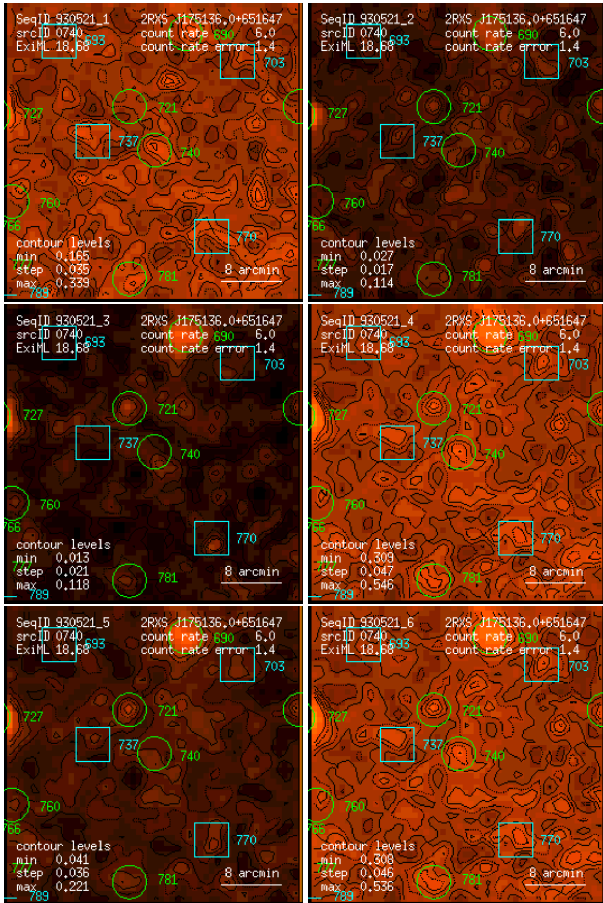
Figure 740: RASS 930521: detection 0740: band rate images, Gaussian filter: (1) PSPC channels 11 – 41, (2) 52 – 90, (3) 91 – 201, (4) 11 – 235, (5) 52 – 201, (6) 11 – 201. Broad band rates in counts/ks. Band rate contour levels in counts/ks/arcmin 2 .
