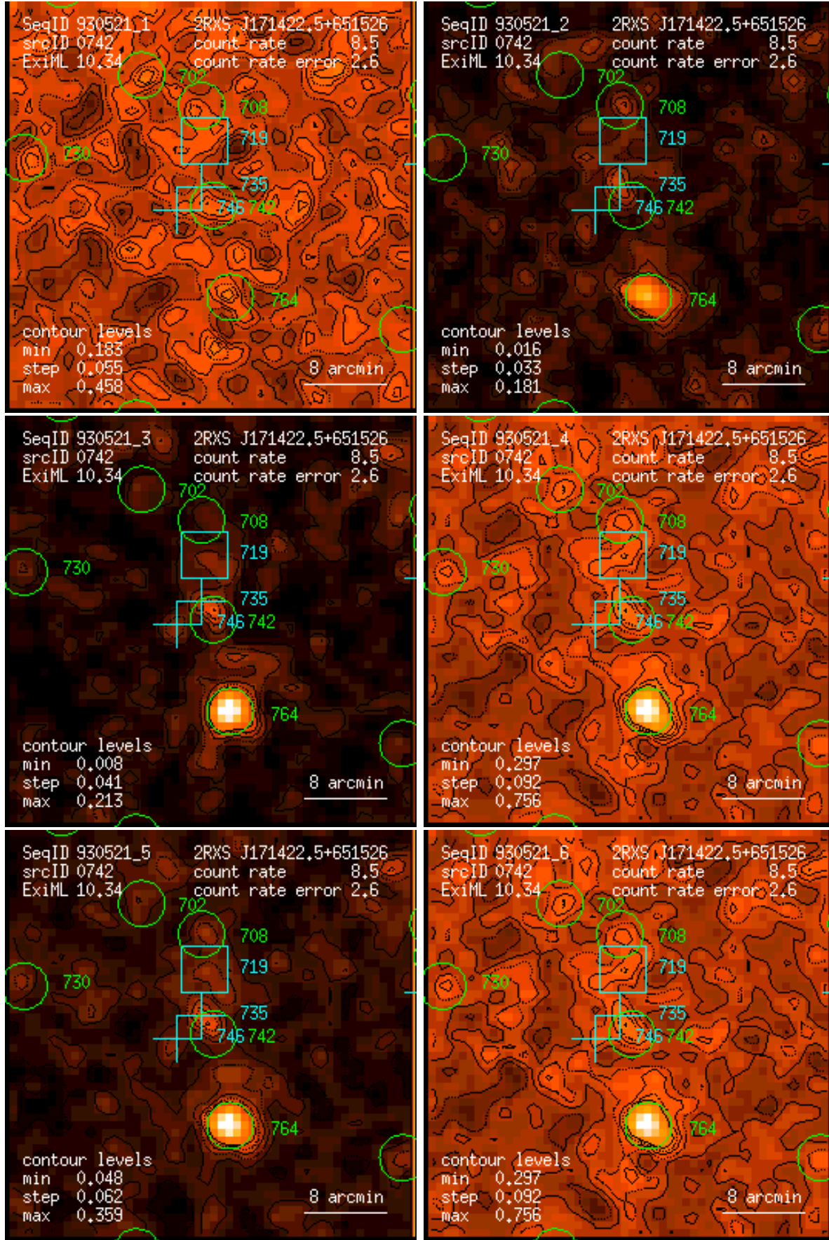
Figure 742: RASS 930521: detection 0742: band rate images, Gaussian filter: (1) PSPC channels 11 – 41, (2) 52 – 90, (3) 91 – 201, (4) 11 – 235, (5) 52 – 201, (6) 11 – 201. Broad band rates in counts/ks. Band rate contour levels in counts/ks/arcmin 2 .
