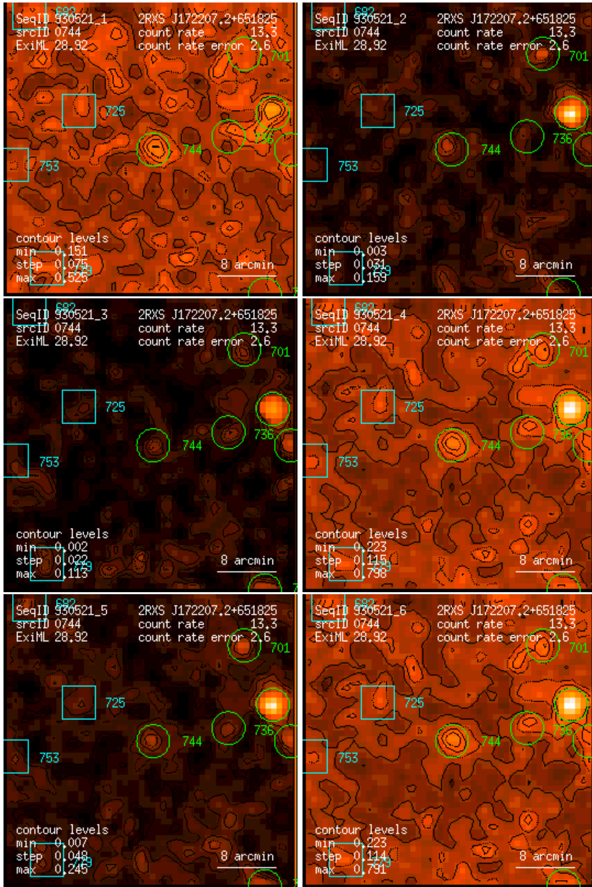
Figure 744: RASS 930521: detection 0744: band rate images, Gaussian filter: (1) PSPC channels 11 – 41, (2) 52 – 90, (3) 91 – 201, (4) 11 – 235, (5) 52 – 201, (6) 11 – 201. Broad band rates in counts/ks. Band rate contour levels in counts/ks/arcmin 2 .
