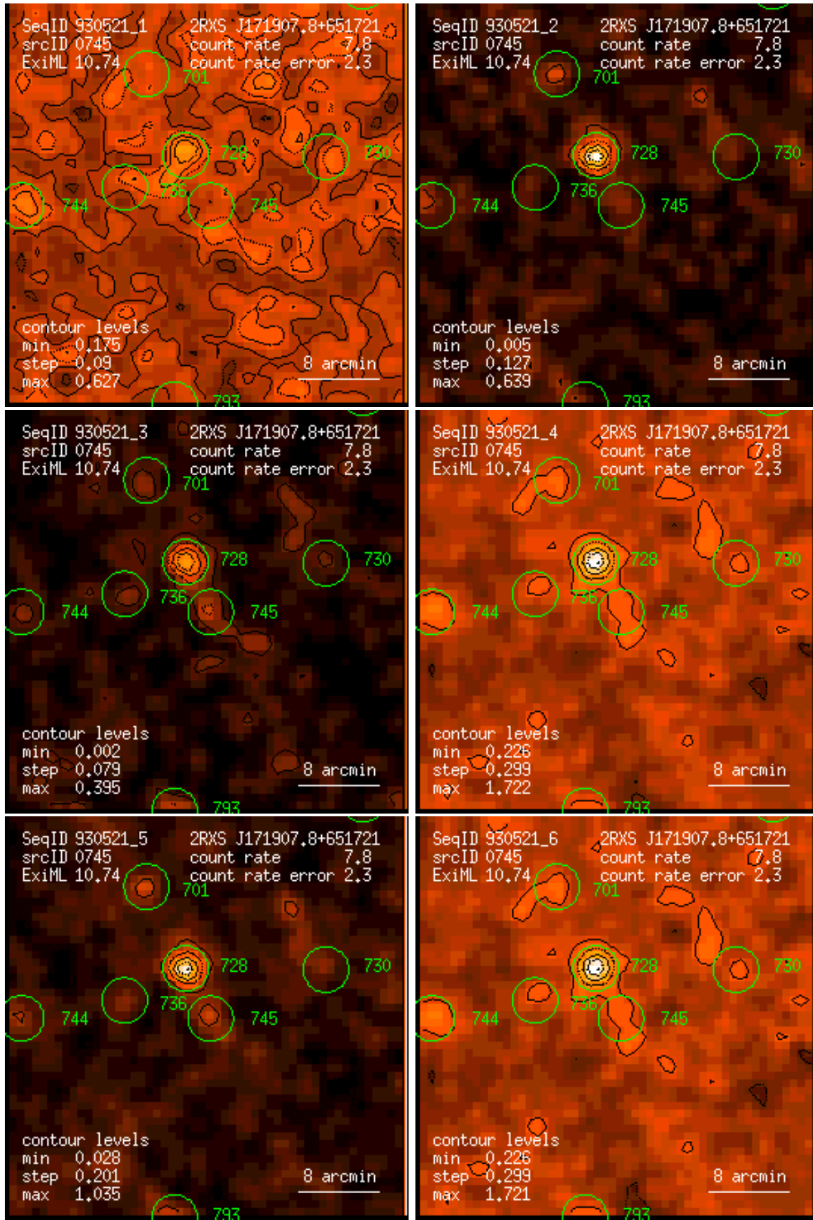
Figure 745: RASS 930521: detection 0745: band rate images, Gaussian filter: (1) PSPC channels 11 – 41, (2) 52 – 90, (3) 91 – 201, (4) 11 – 235, (5) 52 – 201, (6) 11 – 201. Broad band rates in counts/ks. Band rate contour levels in counts/ks/arcmin 2 .
