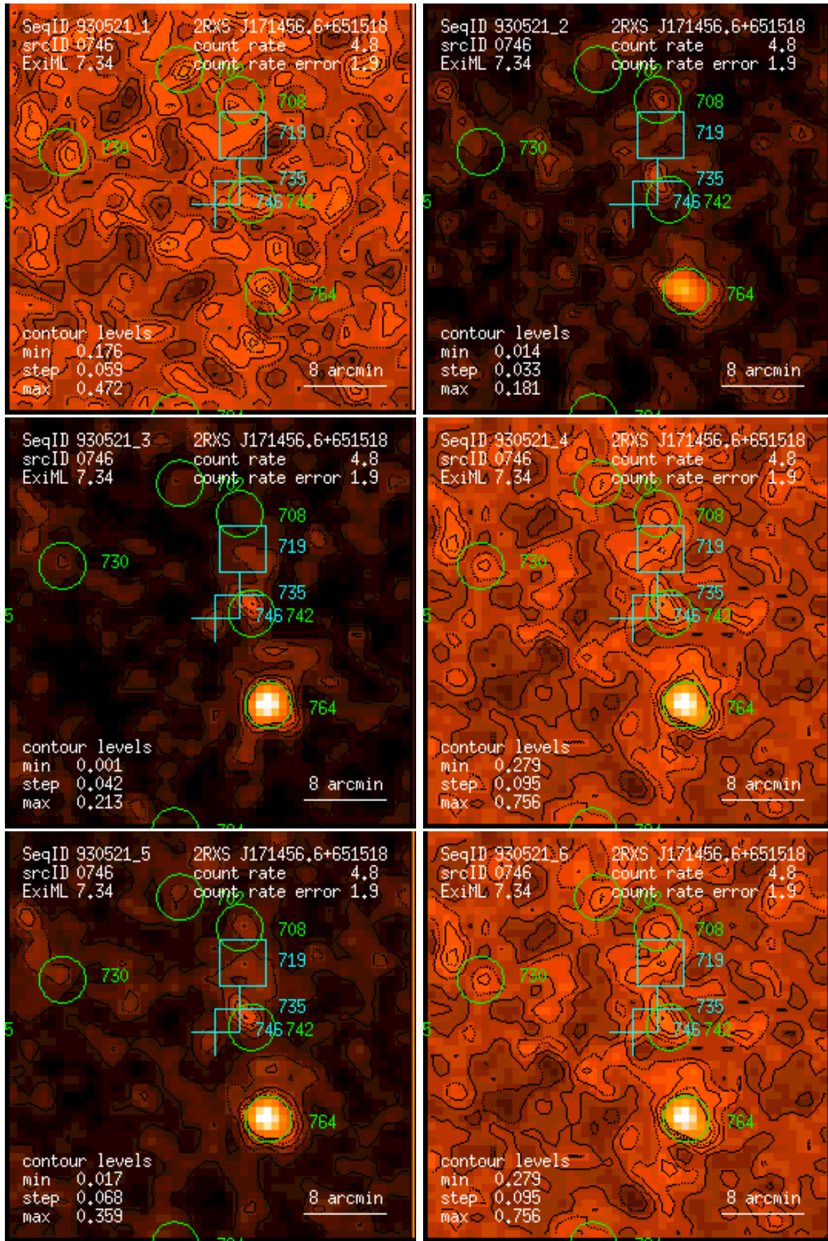
Figure 746: RASS 930521: detection 0746: band rate images, Gaussian filter: (1) PSPC channels 11 – 41, (2) 52 – 90, (3) 91 – 201, (4) 11 – 235, (5) 52 – 201, (6) 11 – 201. Broad band rates in counts/ks. Band rate contour levels in counts/ks/arcmin 2 .
