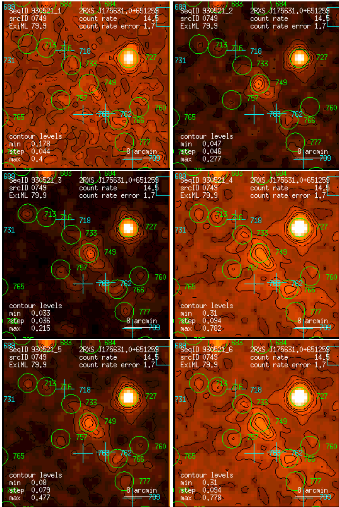
Figure 749: RASS 930521: detection 0749: band rate images, Gaussian filter: (1) PSPC channels 11 – 41, (2) 52 – 90, (3) 91 – 201, (4) 11 – 235, (5) 52 – 201, (6) 11 – 201. Broad band rates in counts/ks. Band rate contour levels in counts/ks/arcmin 2 .
