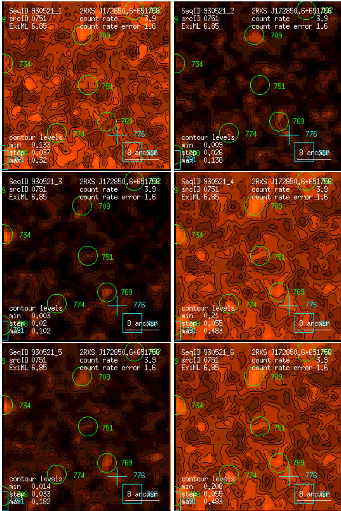
Figure 751: RASS 930521: detection 0751: band rate images, Gaussian filter: (1) PSPC channels 11 – 41, (2) 52 – 90, (3) 91 – 201, (4) 11 – 235, (5) 52 – 201, (6) 11 – 201. Broad band rates in counts/ks. Band rate contour levels in counts/ks/arcmin 2 .
