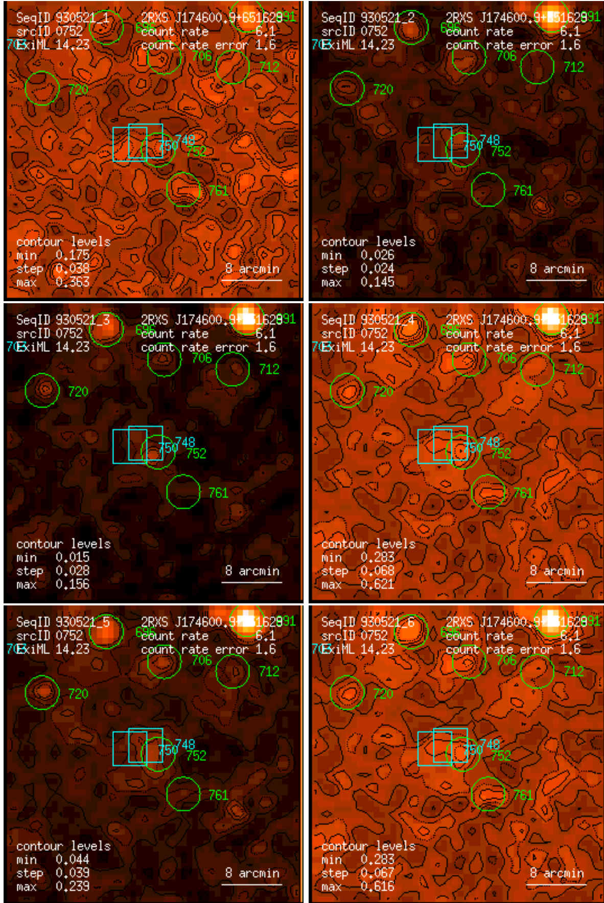
Figure 752: RASS 930521: detection 0752: band rate images, Gaussian filter: (1) PSPC channels 11 – 41, (2) 52 – 90, (3) 91 – 201, (4) 11 – 235, (5) 52 – 201, (6) 11 – 201. Broad band rates in counts/ks. Band rate contour levels in counts/ks/arcmin 2 .
