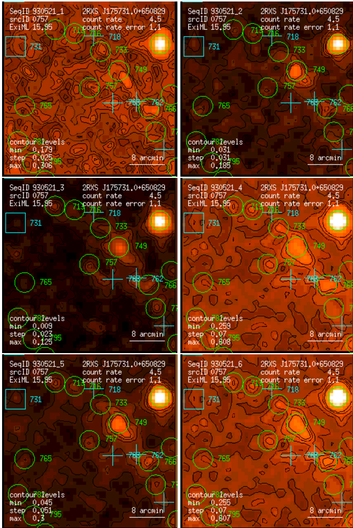
Figure 757: RASS 930521: detection 0757: band rate images, Gaussian filter: (1) PSPC channels 11 – 41, (2) 52 – 90, (3) 91 – 201, (4) 11 – 235, (5) 52 – 201, (6) 11 – 201. Broad band rates in counts/ks. Band rate contour levels in counts/ks/arcmin 2 .
