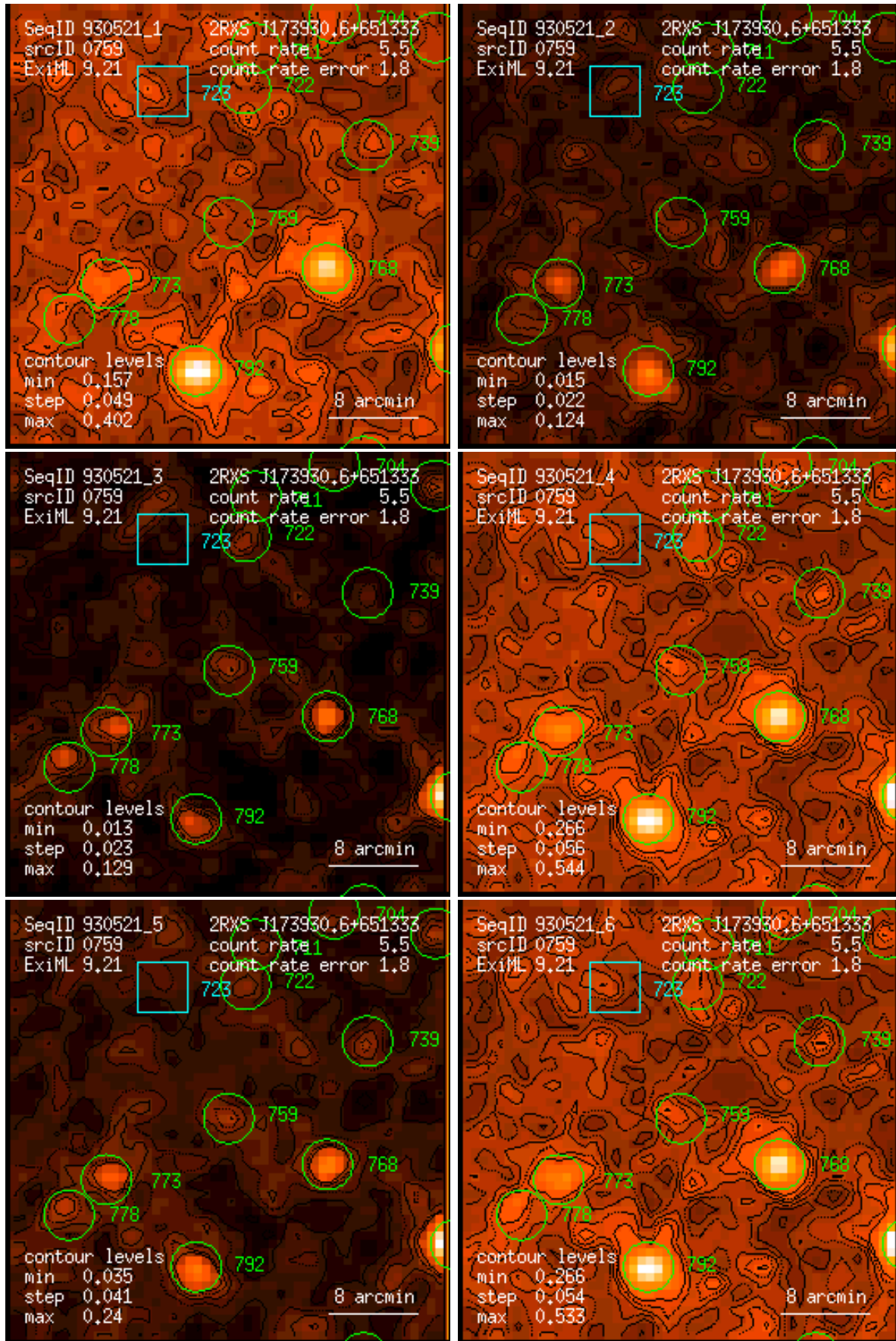
Figure 759: RASS 930521: detection 0759: band rate images, Gaussian filter: (1) PSPC channels 11 – 41, (2) 52 – 90, (3) 91 – 201, (4) 11 – 235, (5) 52 – 201, (6) 11 – 201. Broad band rates in counts/ks. Band rate contour levels in counts/ks/arcmin 2 .
