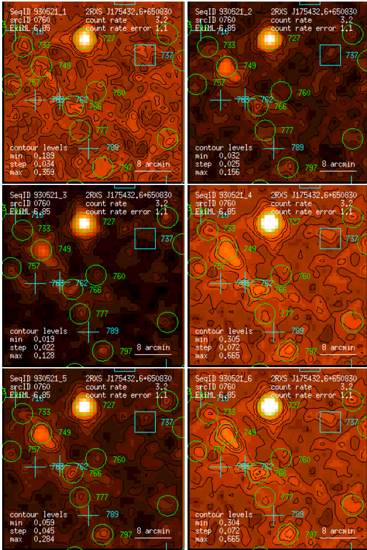
Figure 760: RASS 930521: detection 0760: band rate images, Gaussian filter: (1) PSPC channels 11 – 41, (2) 52 – 90, (3) 91 – 201, (4) 11 – 235, (5) 52 – 201, (6) 11 – 201. Broad band rates in counts/ks. Band rate contour levels in counts/ks/arcmin 2 .
