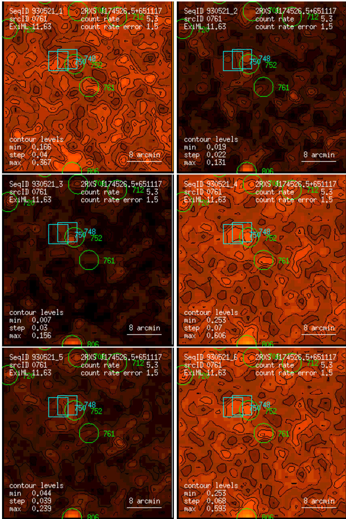
Figure 761: RASS 930521: detection 0761: band rate images, Gaussian filter: (1) PSPC channels 11 – 41, (2) 52 – 90, (3) 91 – 201, (4) 11 – 235, (5) 52 – 201, (6) 11 – 201. Broad band rates in counts/ks. Band rate contour levels in counts/ks/arcmin 2 .
