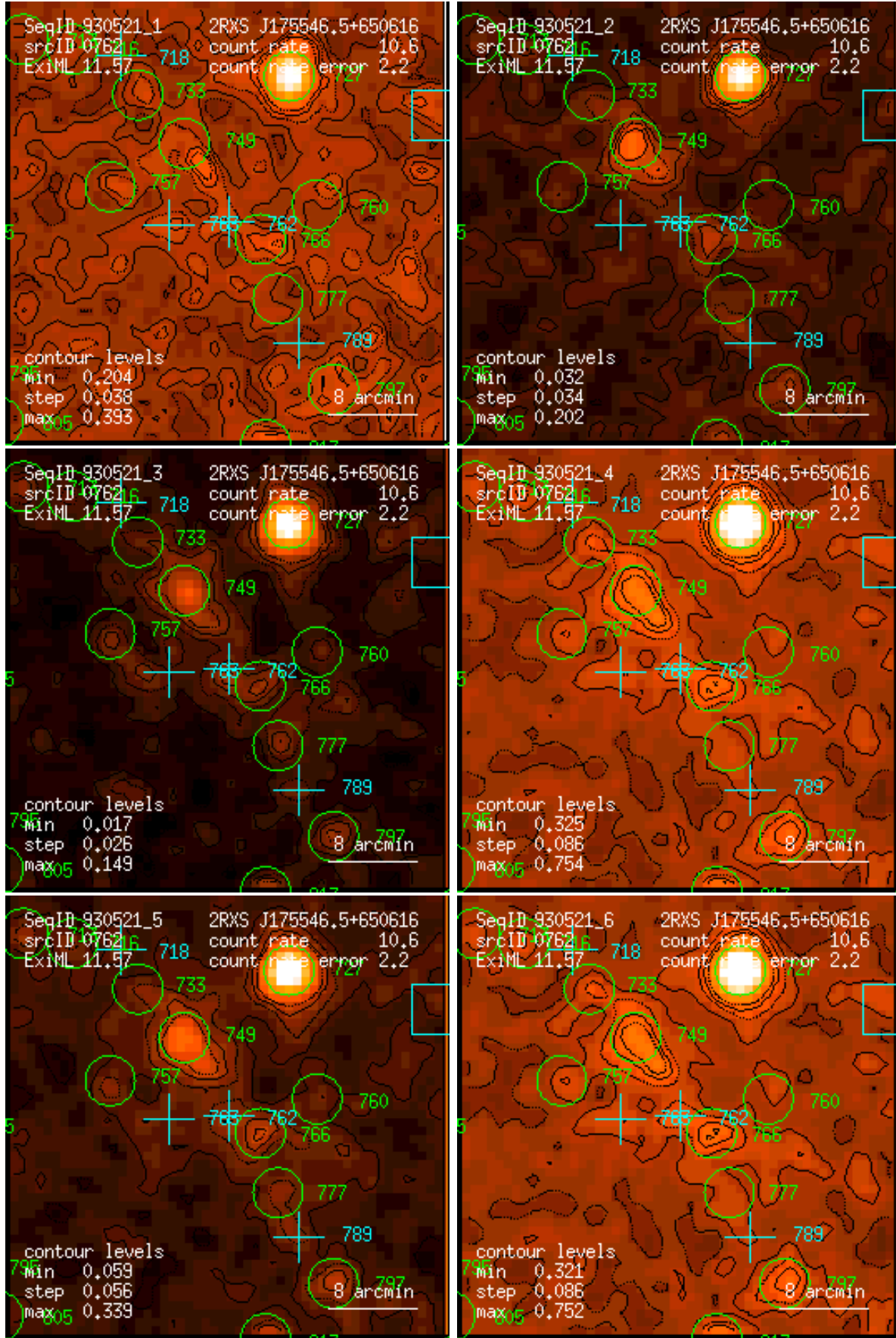
Figure 762: RASS 930521: detection 0762: band rate images, Gaussian filter: (1) PSPC channels 11 – 41, (2) 52 – 90, (3) 91 – 201, (4) 11 – 235, (5) 52 – 201, (6) 11 – 201. Broad band rates in counts/ks. Band rate contour levels in counts/ks/arcmin 2 .
