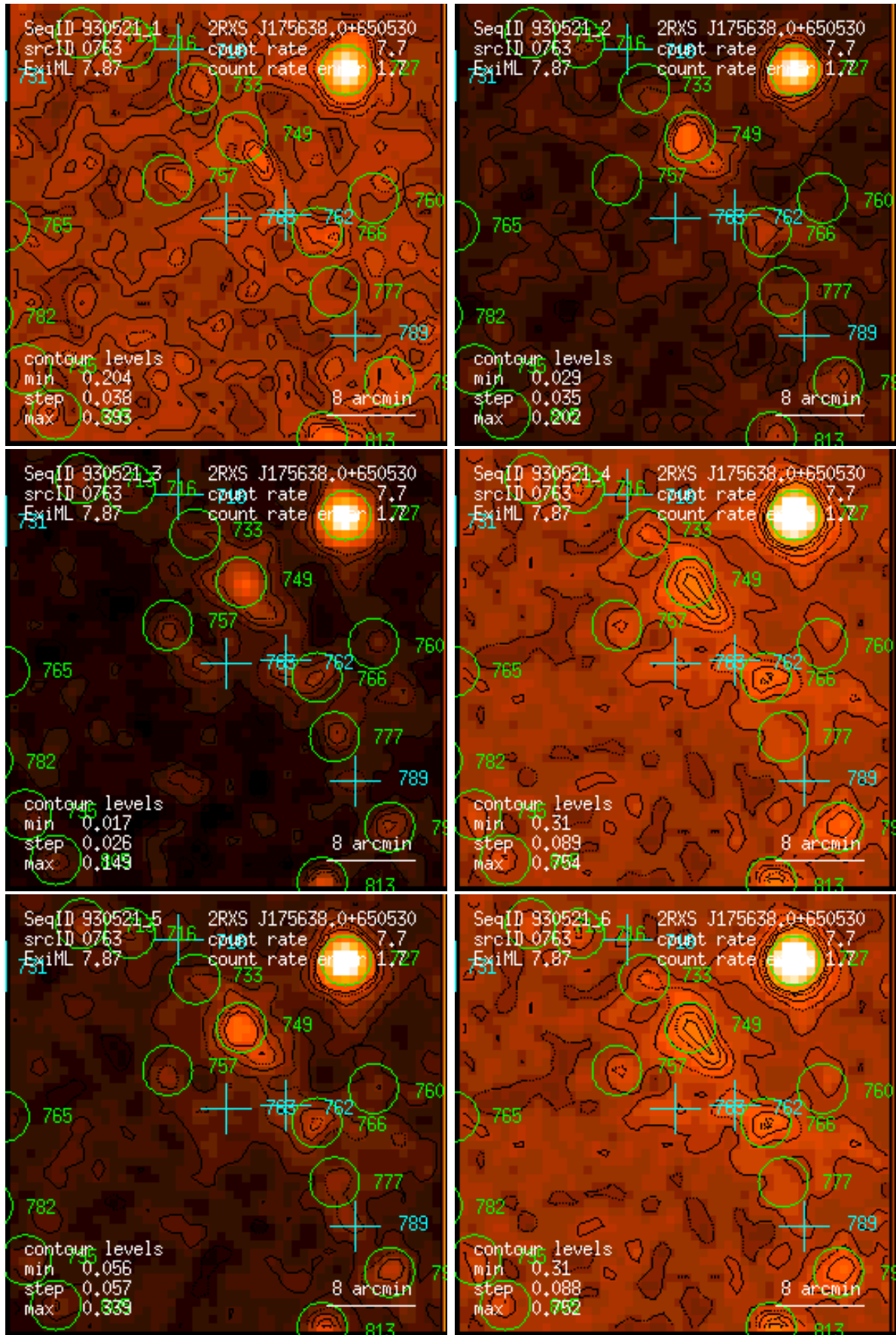
Figure 763: RASS 930521: detection 0763: band rate images, Gaussian filter: (1) PSPC channels 11 – 41, (2) 52 – 90, (3) 91 – 201, (4) 11 – 235, (5) 52 – 201, (6) 11 – 201. Broad band rates in counts/ks. Band rate contour levels in counts/ks/arcmin 2 .
