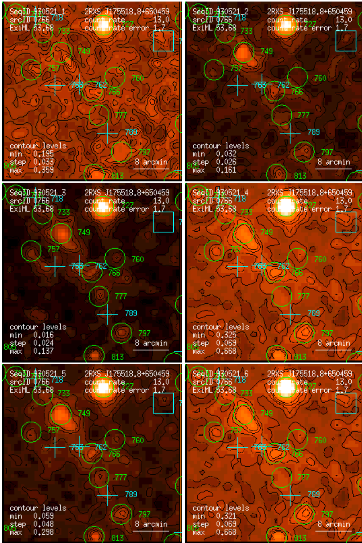
Figure 766: RASS 930521: detection 0766: band rate images, Gaussian filter: (1) PSPC channels 11 – 41, (2) 52 – 90, (3) 91 – 201, (4) 11 – 235, (5) 52 – 201, (6) 11 – 201. Broad band rates in counts/ks. Band rate contour levels in counts/ks/arcmin 2 .
