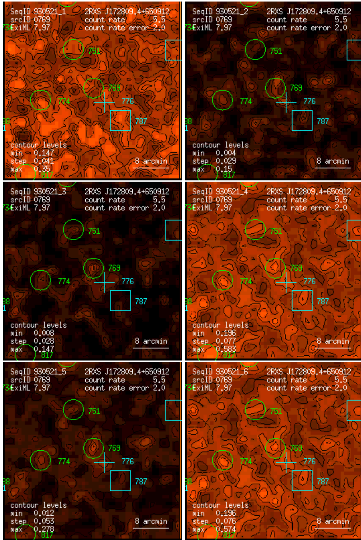
Figure 769: RASS 930521: detection 0769: band rate images, Gaussian filter: (1) PSPC channels 11 – 41, (2) 52 – 90, (3) 91 – 201, (4) 11 – 235, (5) 52 – 201, (6) 11 – 201. Broad band rates in counts/ks. Band rate contour levels in counts/ks/arcmin 2 .
