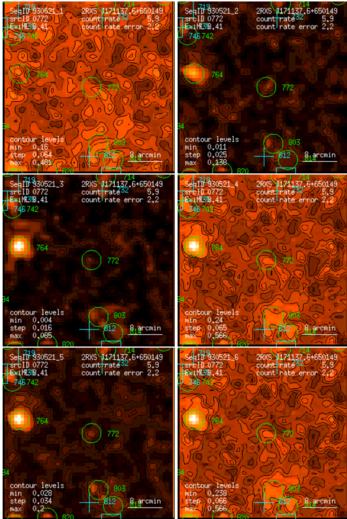
Figure 772: RASS 930521: detection 0772: band rate images, Gaussian filter: (1) PSPC channels 11 – 41, (2) 52 – 90, (3) 91 – 201, (4) 11 – 235, (5) 52 – 201, (6) 11 – 201. Broad band rates in counts/ks. Band rate contour levels in counts/ks/arcmin 2 .
