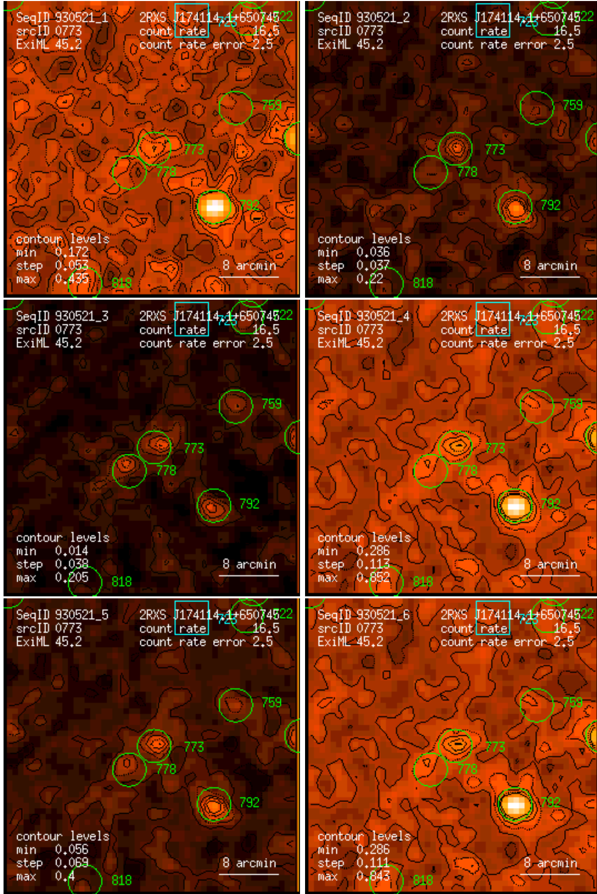
Figure 773: RASS 930521: detection 0773: band rate images, Gaussian filter: (1) PSPC channels 11 – 41, (2) 52 – 90, (3) 91 – 201, (4) 11 – 235, (5) 52 – 201, (6) 11 – 201. Broad band rates in counts/ks. Band rate contour levels in counts/ks/arcmin 2 .
