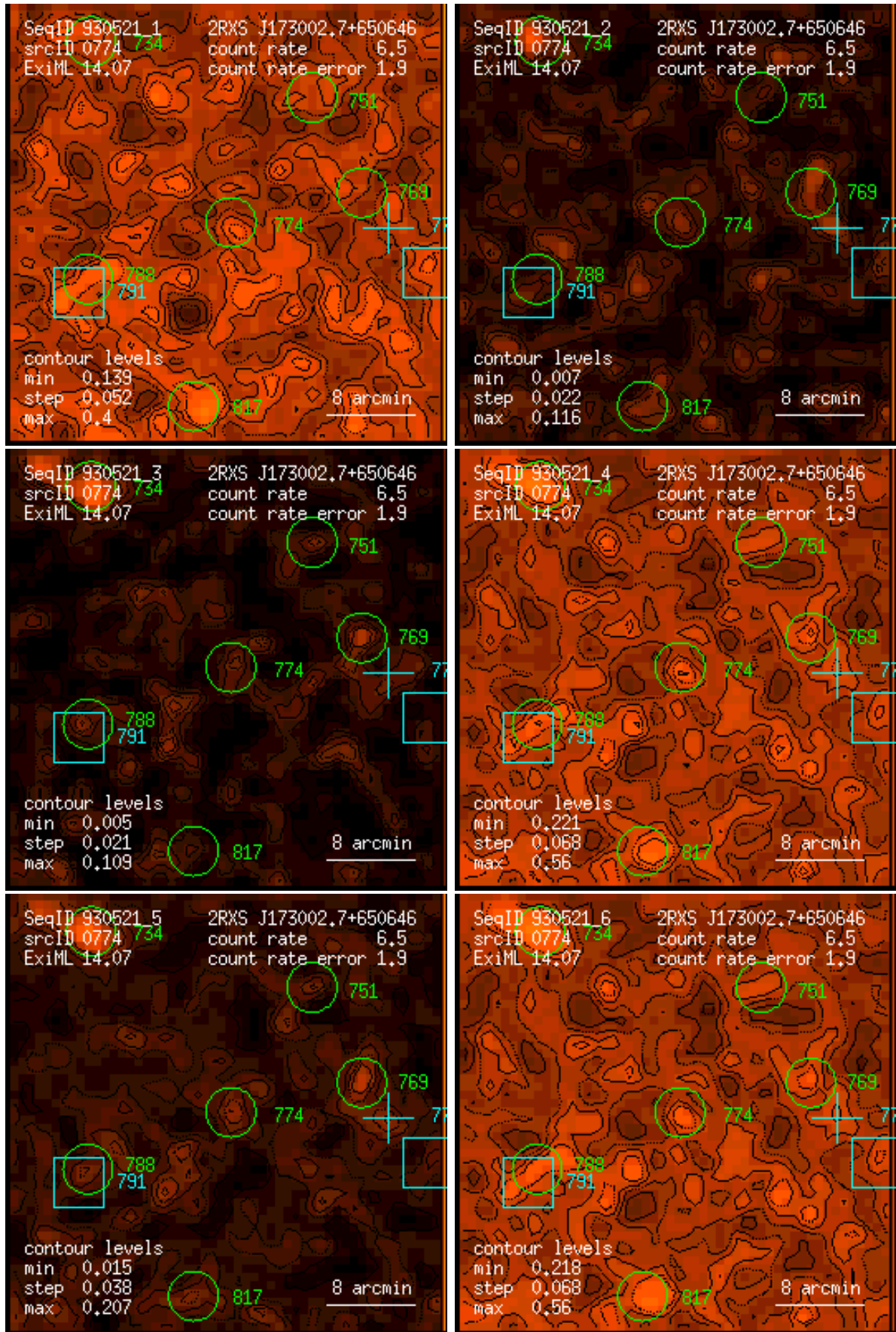
Figure 774: RASS 930521: detection 0774: band rate images, Gaussian filter: (1) PSPC channels 11 – 41, (2) 52 – 90, (3) 91 – 201, (4) 11 – 235, (5) 52 – 201, (6) 11 – 201. Broad band rates in counts/ks. Band rate contour levels in counts/ks/arcmin 2 .
