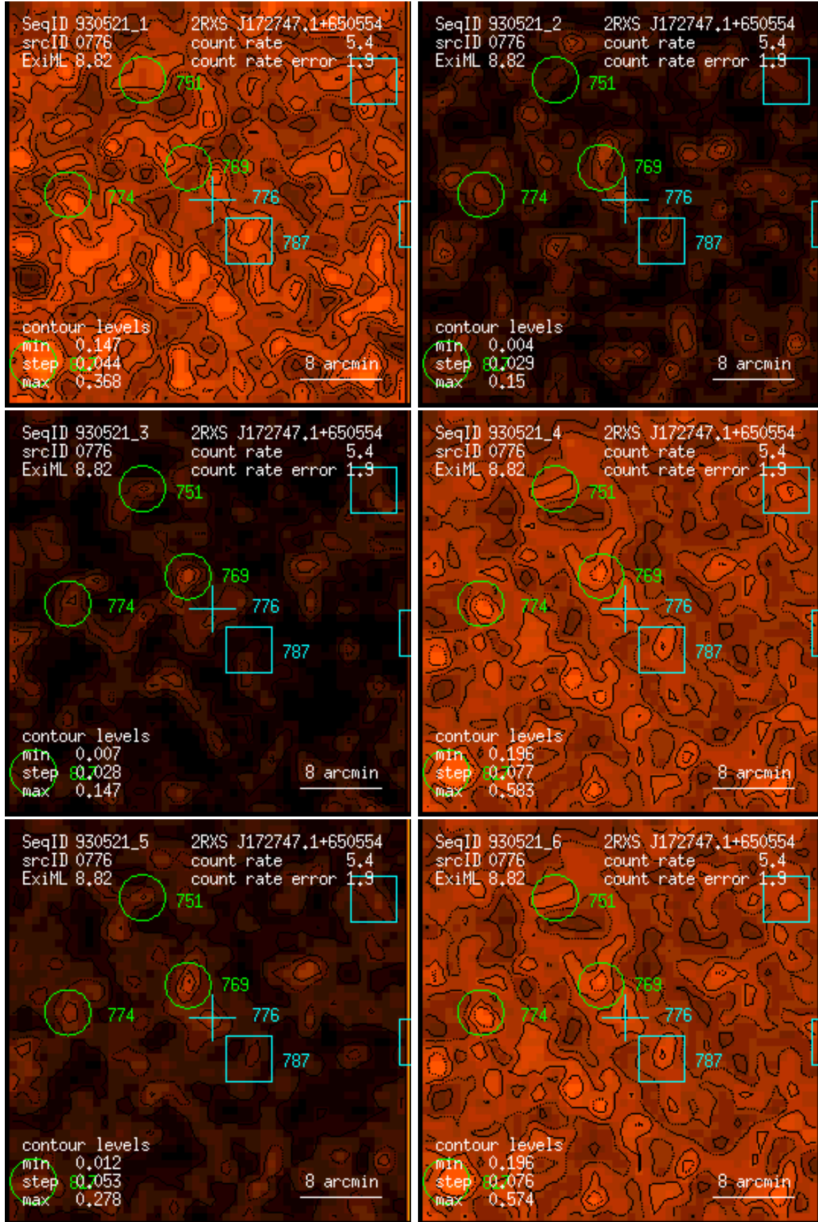
Figure 776: RASS 930521: detection 0776: band rate images, Gaussian filter: (1) PSPC channels 11 – 41, (2) 52 – 90, (3) 91 – 201, (4) 11 – 235, (5) 52 – 201, (6) 11 – 201. Broad band rates in counts/ks. Band rate contour levels in counts/ks/arcmin 2 .
