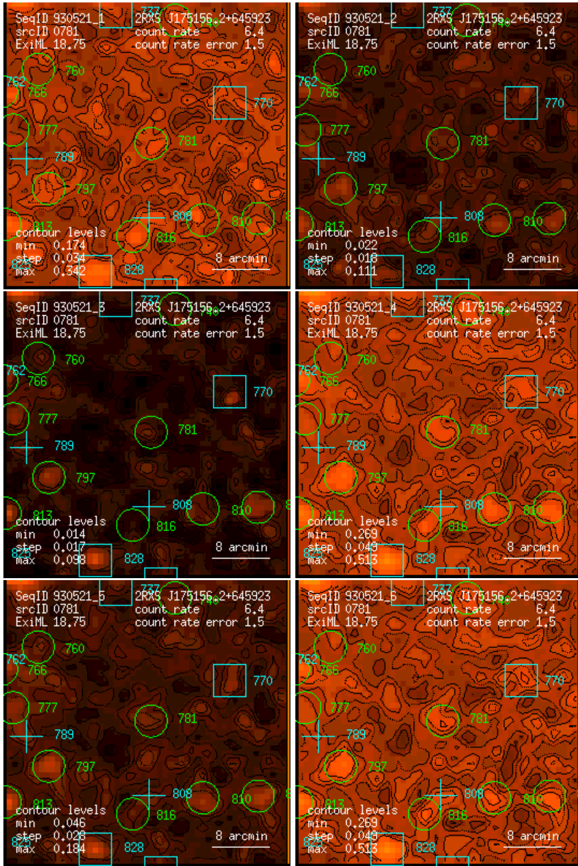
Figure 781: RASS 930521: detection 0781: band rate images, Gaussian filter: (1) PSPC channels 11 – 41, (2) 52 – 90, (3) 91 – 201, (4) 11 – 235, (5) 52 – 201, (6) 11 – 201. Broad band rates in counts/ks. Band rate contour levels in counts/ks/arcmin 2 .
