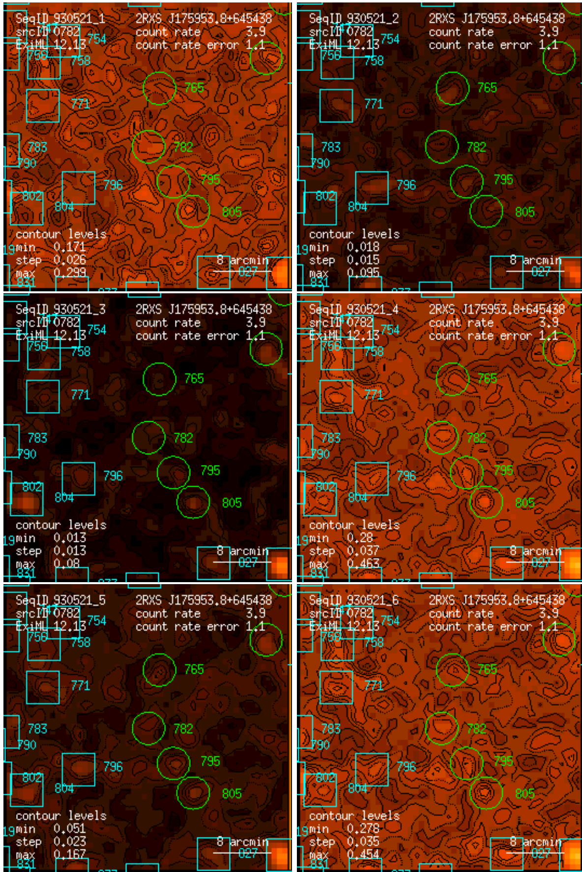
Figure 782: RASS 930521: detection 0782: band rate images, Gaussian filter: (1) PSPC channels 11 – 41, (2) 52 – 90, (3) 91 – 201, (4) 11 – 235, (5) 52 – 201, (6) 11 – 201. Broad band rates in counts/ks. Band rate contour levels in counts/ks/arcmin 2 .
