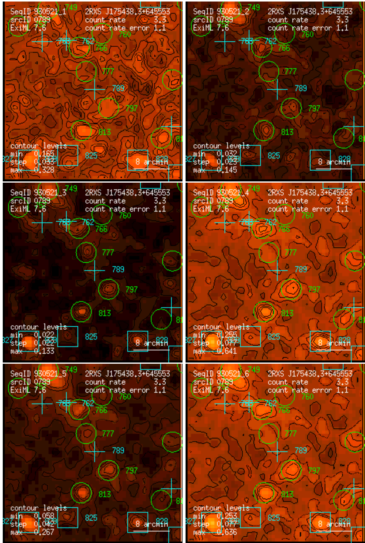
Figure 789: RASS 930521: detection 0789: band rate images, Gaussian filter: (1) PSPC channels 11 – 41, (2) 52 – 90, (3) 91 – 201, (4) 11 – 235, (5) 52 – 201, (6) 11 – 201. Broad band rates in counts/ks. Band rate contour levels in counts/ks/arcmin 2 .
