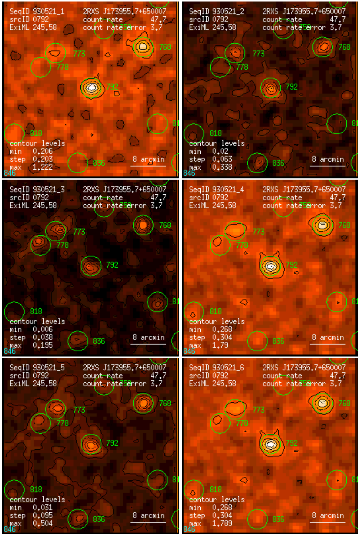
Figure 792: RASS 930521: detection 0792: band rate images, Gaussian filter: (1) PSPC channels 11 – 41, (2) 52 – 90, (3) 91 – 201, (4) 11 – 235, (5) 52 – 201, (6) 11 – 201. Broad band rates in counts/ks. Band rate contour levels in counts/ks/arcmin 2 .
