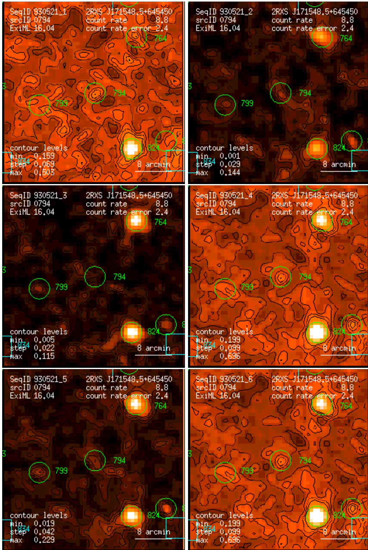
Figure 794: RASS 930521: detection 0794: band rate images, Gaussian filter: (1) PSPC channels 11 – 41, (2) 52 – 90, (3) 91 – 201, (4) 11 – 235, (5) 52 – 201, (6) 11 – 201. Broad band rates in counts/ks. Band rate contour levels in counts/ks/arcmin 2 .
