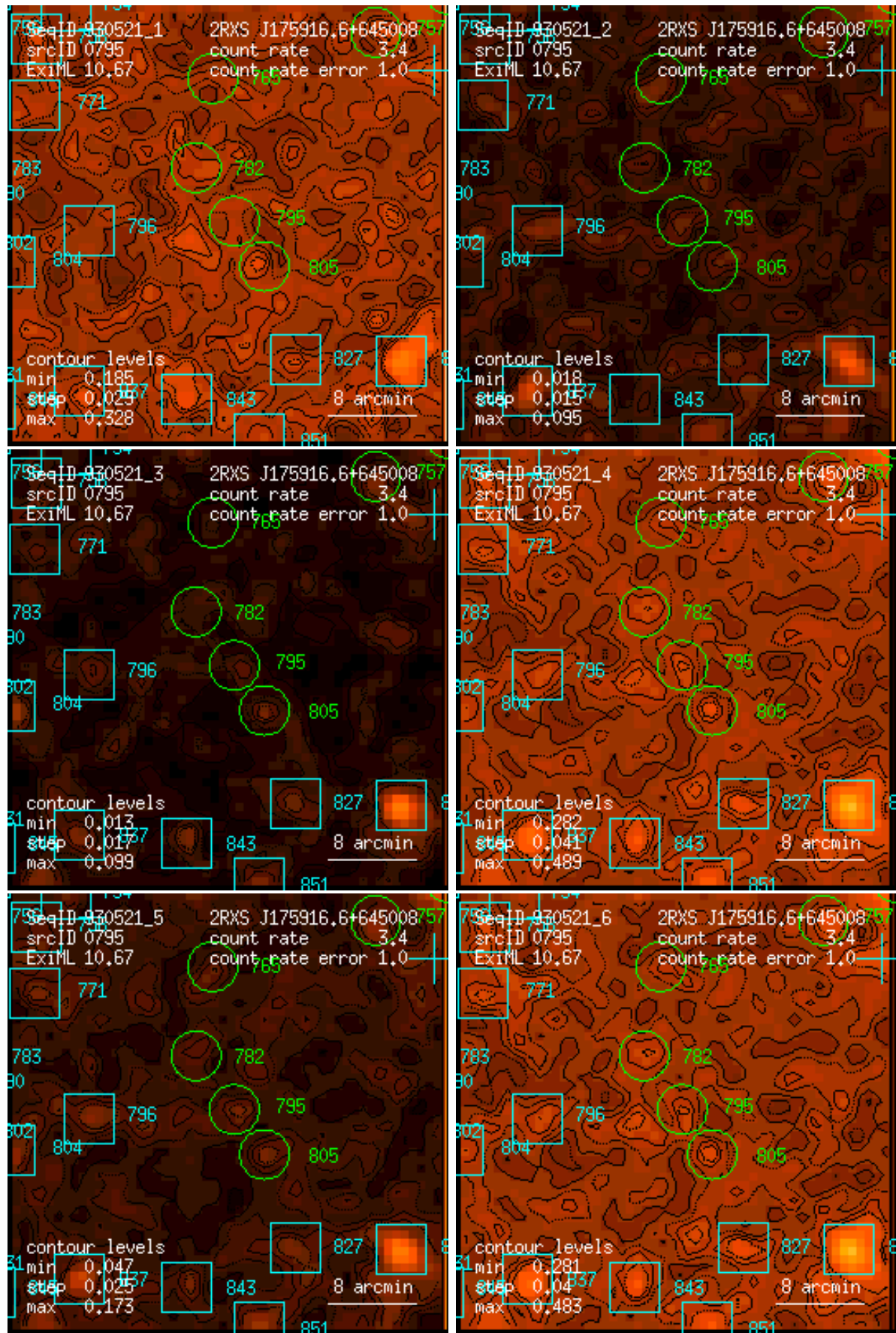
Figure 795: RASS 930521: detection 0795: band rate images, Gaussian filter: (1) PSPC channels 11 – 41, (2) 52 – 90, (3) 91 – 201, (4) 11 – 235, (5) 52 – 201, (6) 11 – 201. Broad band rates in counts/ks. Band rate contour levels in counts/ks/arcmin 2 .
