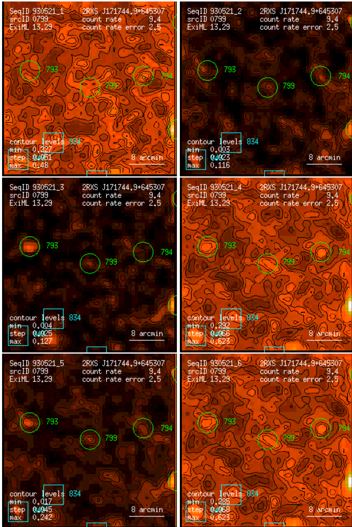
Figure 799: RASS 930521: detection 0799: band rate images, Gaussian filter: (1) PSPC channels 11 – 41, (2) 52 – 90, (3) 91 – 201, (4) 11 – 235, (5) 52 – 201, (6) 11 – 201. Broad band rates in counts/ks. Band rate contour levels in counts/ks/arcmin 2 .
