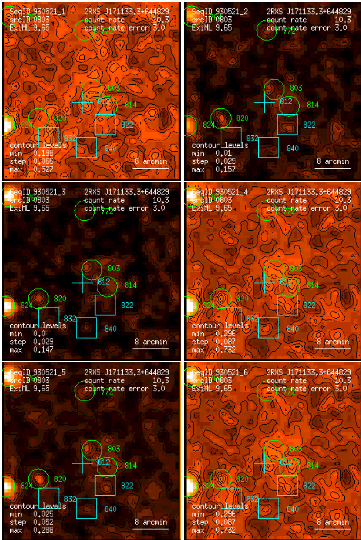
Figure 803: RASS 930521: detection 0803: band rate images, Gaussian filter: (1) PSPC channels 11 – 41, (2) 52 – 90, (3) 91 – 201, (4) 11 – 235, (5) 52 – 201, (6) 11 – 201. Broad band rates in counts/ks. Band rate contour levels in counts/ks/arcmin 2 .
