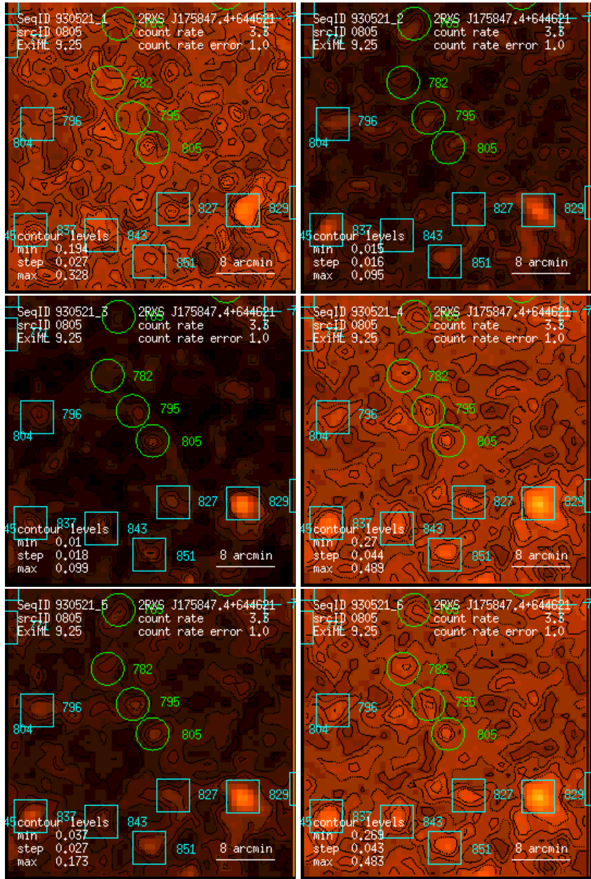
Figure 805: RASS 930521: detection 0805: band rate images, Gaussian filter: (1) PSPC channels 11 – 41, (2) 52 – 90, (3) 91 – 201, (4) 11 – 235, (5) 52 – 201, (6) 11 – 201. Broad band rates in counts/ks. Band rate contour levels in counts/ks/arcmin 2 .
