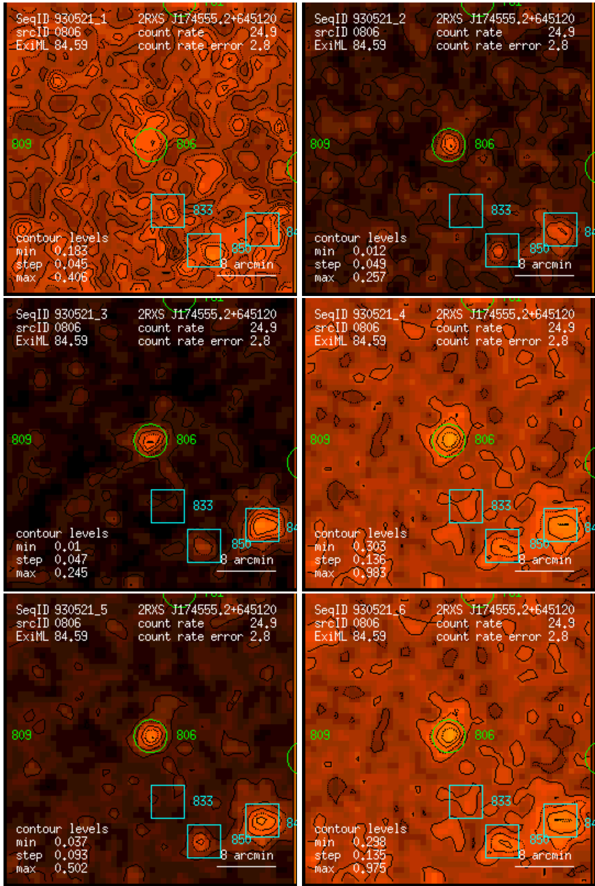
Figure 806: RASS 930521: detection 0806: band rate images, Gaussian filter: (1) PSPC channels 11 – 41, (2) 52 – 90, (3) 91 – 201, (4) 11 – 235, (5) 52 – 201, (6) 11 – 201. Broad band rates in counts/ks. Band rate contour levels in counts/ks/arcmin 2 .
