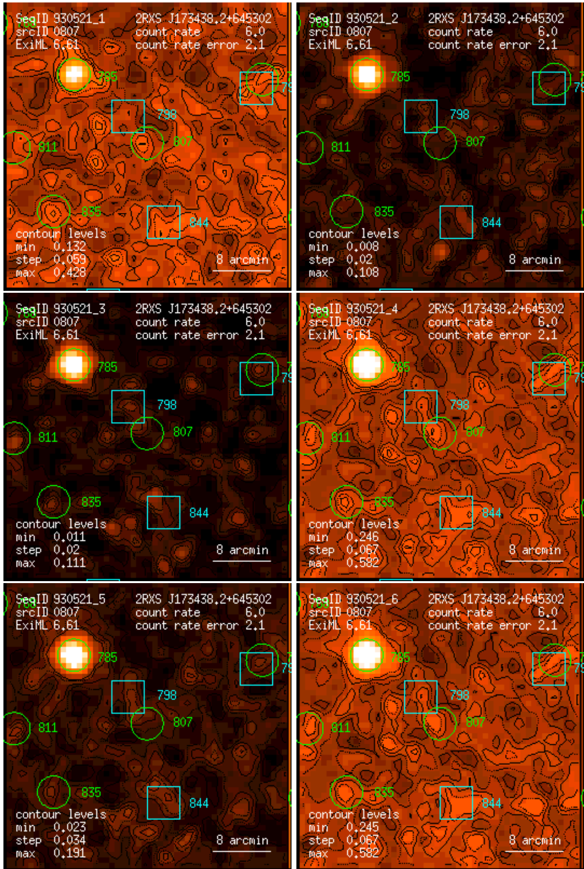
Figure 807: RASS 930521: detection 0807: band rate images, Gaussian filter: (1) PSPC channels 11 – 41, (2) 52 – 90, (3) 91 – 201, (4) 11 – 235, (5) 52 – 201, (6) 11 – 201. Broad band rates in counts/ks. Band rate contour levels in counts/ks/arcmin 2 .
