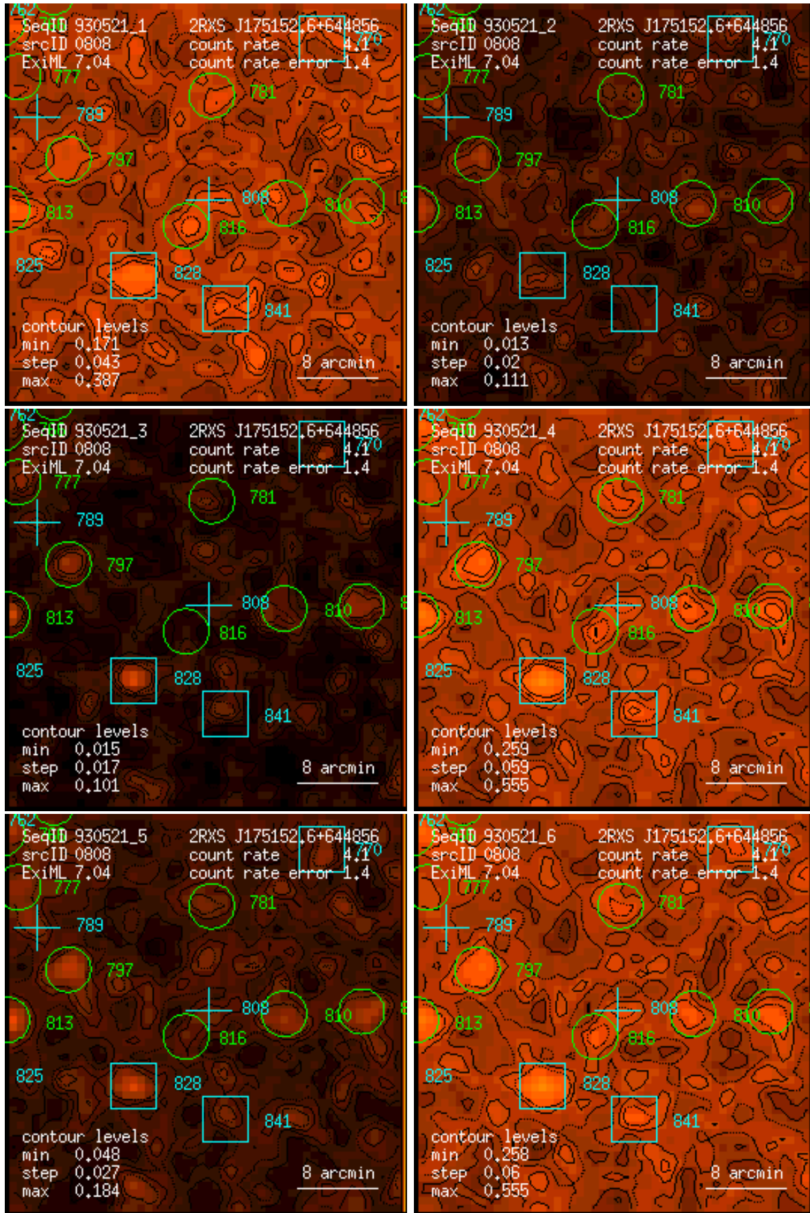
Figure 808: RASS 930521: detection 0808: band rate images, Gaussian filter: (1) PSPC channels 11 – 41, (2) 52 – 90, (3) 91 – 201, (4) 11 – 235, (5) 52 – 201, (6) 11 – 201. Broad band rates in counts/ks. Band rate contour levels in counts/ks/arcmin 2 .
