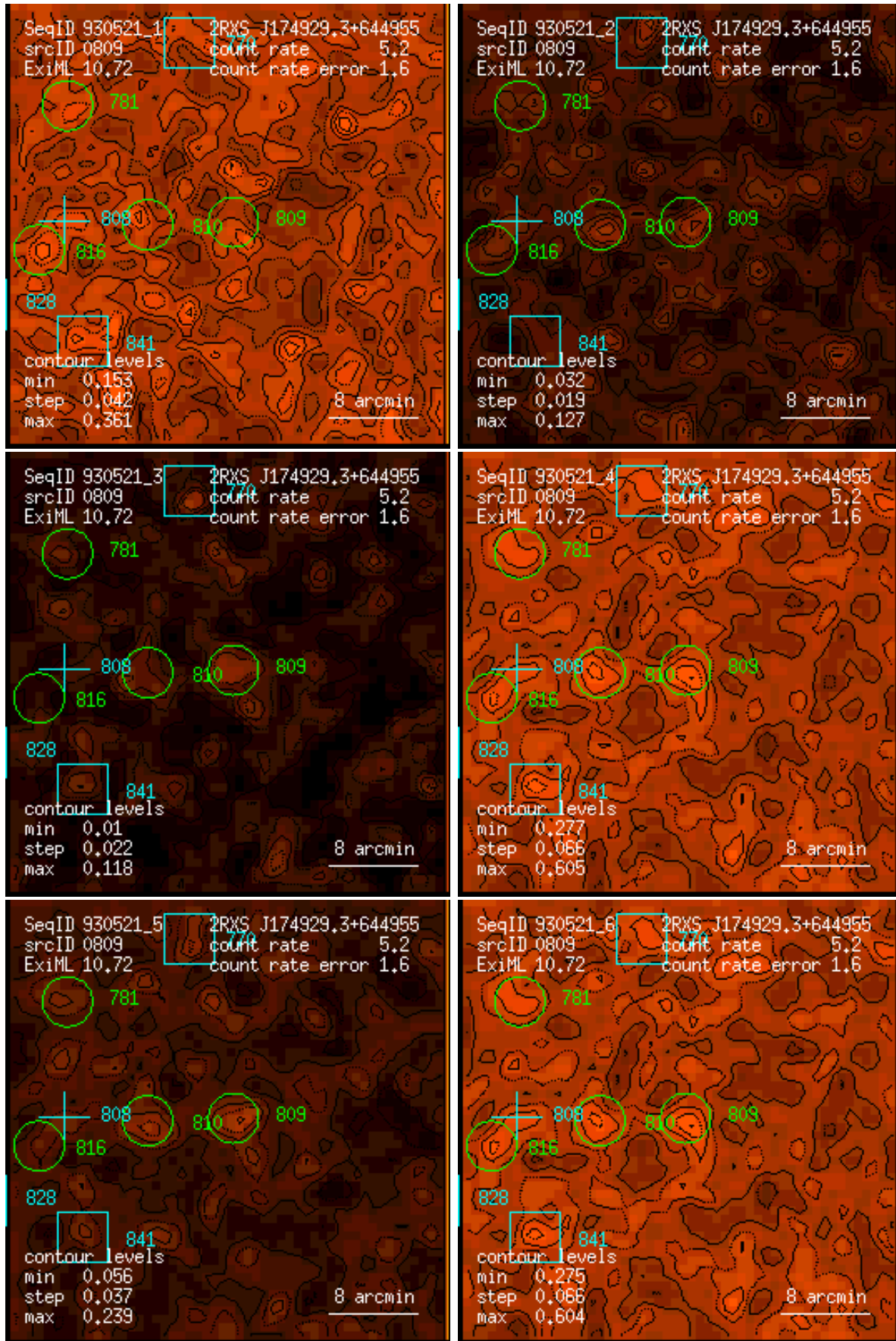
Figure 809: RASS 930521: detection 0809: band rate images, Gaussian filter: (1) PSPC channels 11 – 41, (2) 52 – 90, (3) 91 – 201, (4) 11 – 235, (5) 52 – 201, (6) 11 – 201. Broad band rates in counts/ks. Band rate contour levels in counts/ks/arcmin 2 .
