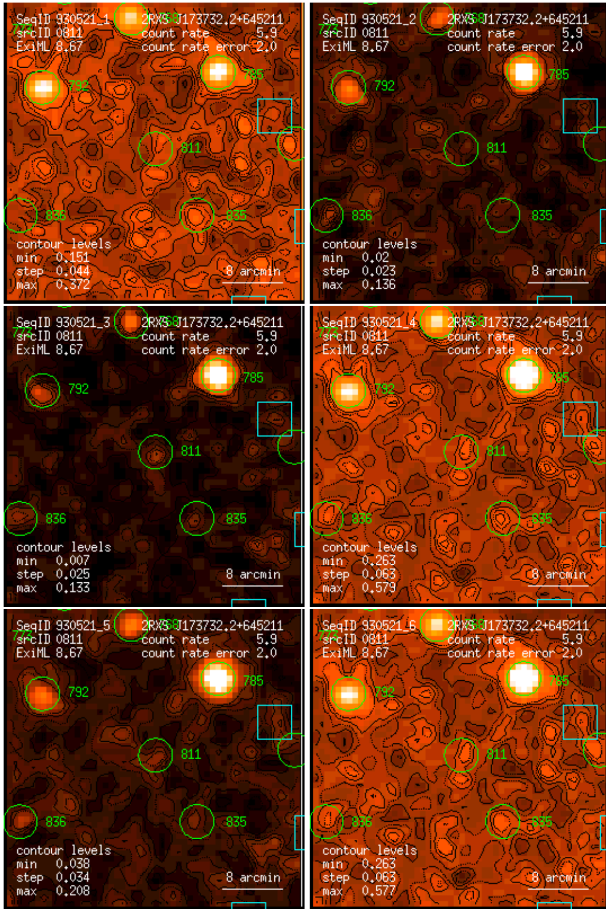
Figure 811: RASS 930521: detection 0811: band rate images, Gaussian filter: (1) PSPC channels 11 – 41, (2) 52 – 90, (3) 91 – 201, (4) 11 – 235, (5) 52 – 201, (6) 11 – 201. Broad band rates in counts/ks. Band rate contour levels in counts/ks/arcmin 2 .
