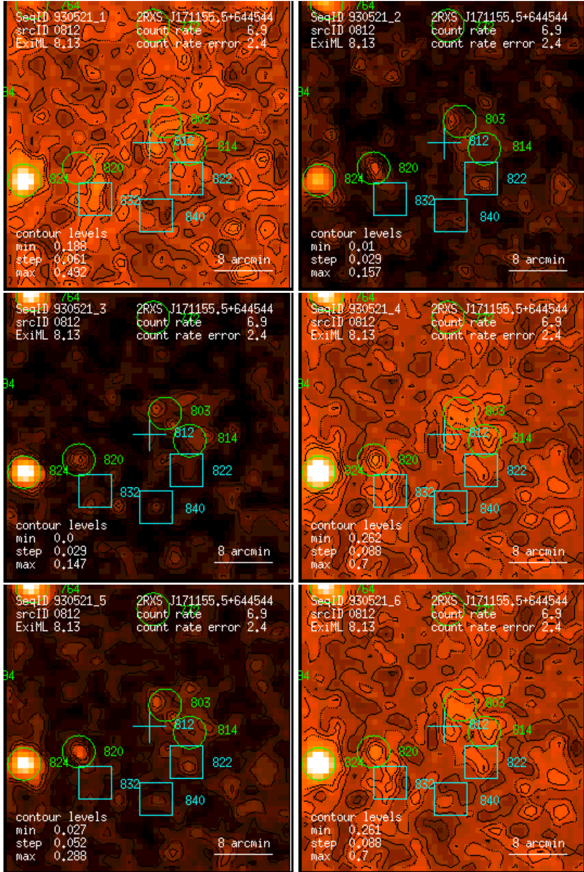
Figure 812: RASS 930521: detection 0812: band rate images, Gaussian filter: (1) PSPC channels 11 – 41, (2) 52 – 90, (3) 91 – 201, (4) 11 – 235, (5) 52 – 201, (6) 11 – 201. Broad band rates in counts/ks. Band rate contour levels in counts/ks/arcmin 2 .
